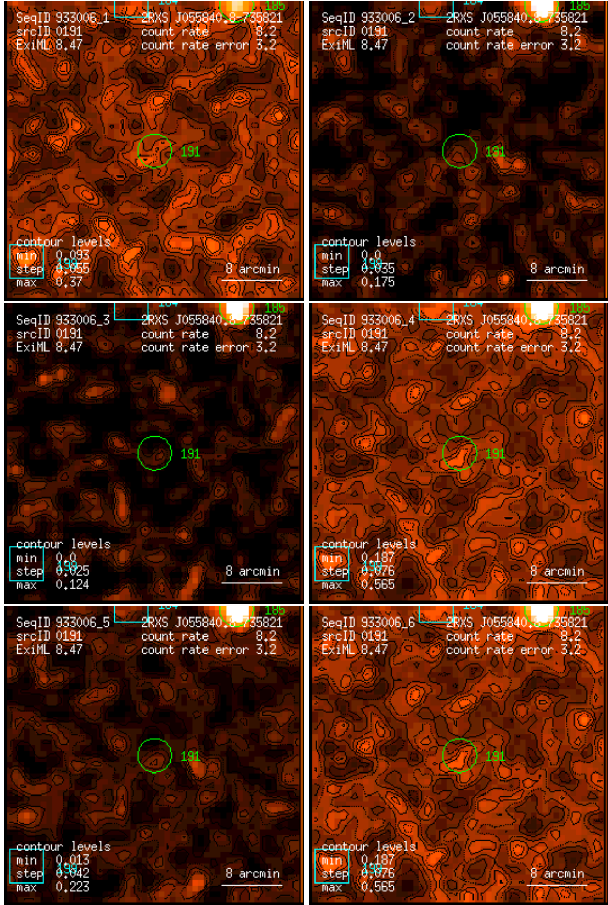
Figure 191: RASS 933006: detection 0191: band rate images, Gaussian filter: (1) PSPC channels 11 – 41, (2) 52 – 90, (3) 91 – 201, (4) 11 – 235, (5) 52 – 201, (6) 11 – 201. Broad band rates in counts/ks. Band rate contour levels in counts/ks/arcmin 2 .
