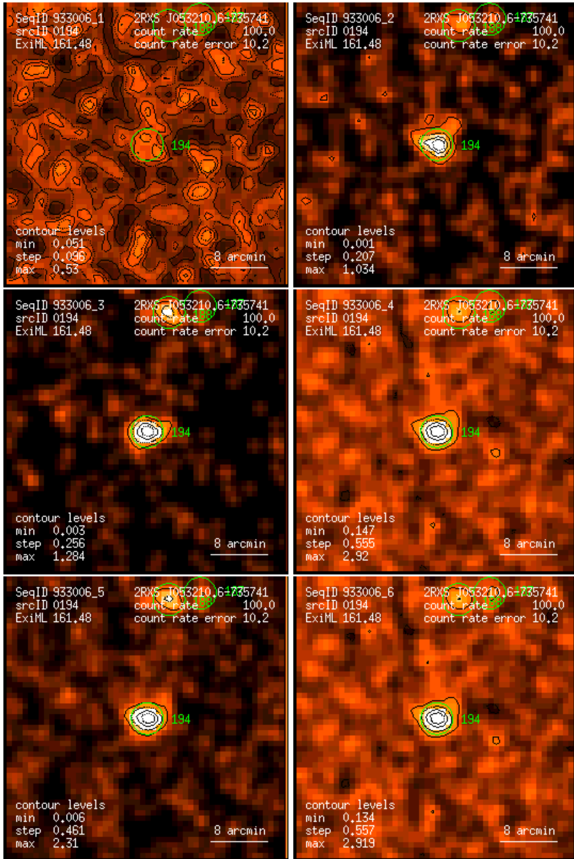
Figure 194: RASS 933006: detection 0194: band rate images, Gaussian filter: (1) PSPC channels 11 – 41, (2) 52 – 90, (3) 91 – 201, (4) 11 – 235, (5) 52 – 201, (6) 11 – 201. Broad band rates in counts/ks. Band rate contour levels in counts/ks/arcmin 2 .
