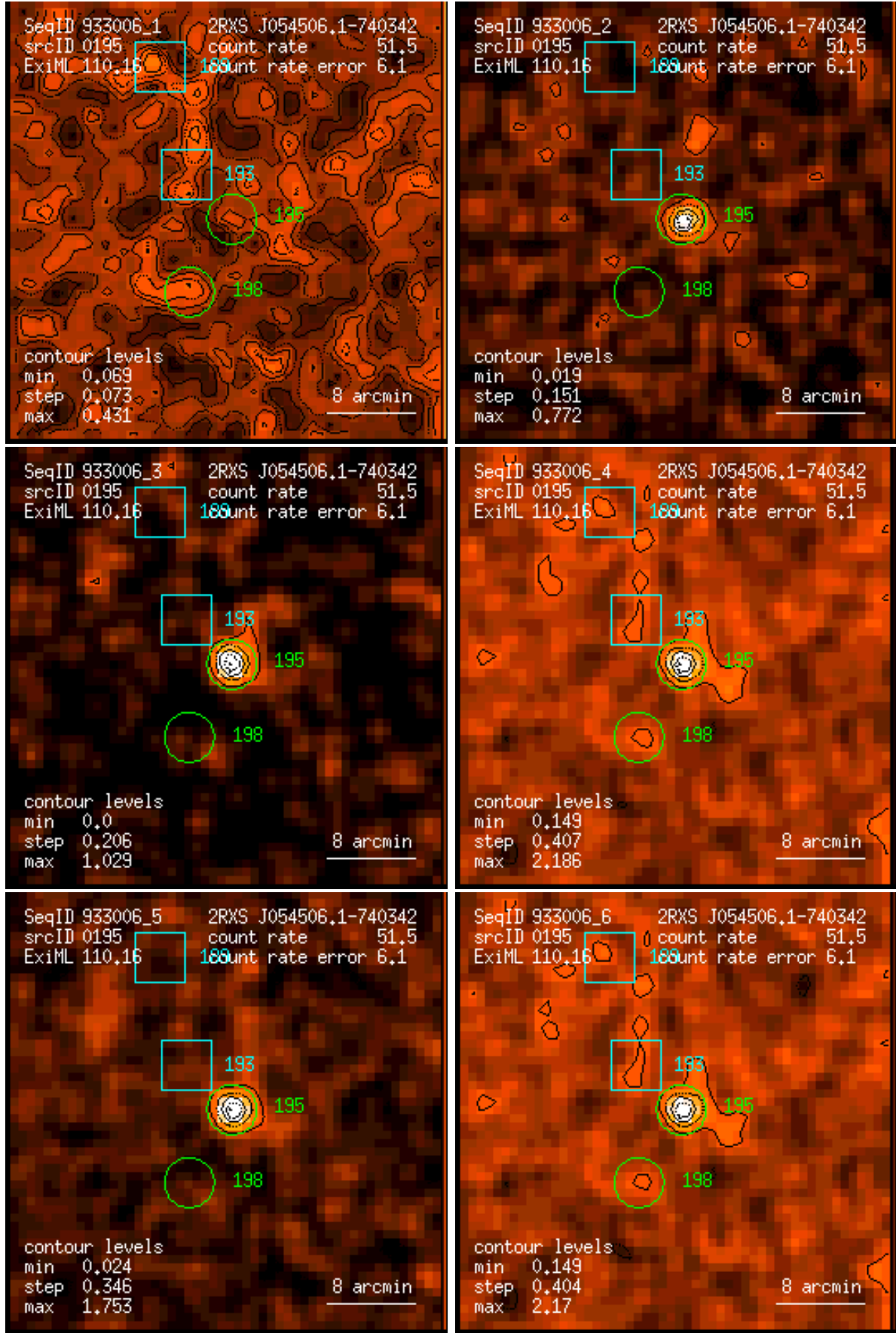
Figure 195: RASS 933006: detection 0195: band rate images, Gaussian filter: (1) PSPC channels 11 – 41, (2) 52 – 90, (3) 91 – 201, (4) 11 – 235, (5) 52 – 201, (6) 11 – 201. Broad band rates in counts/ks. Band rate contour levels in counts/ks/arcmin 2 .
