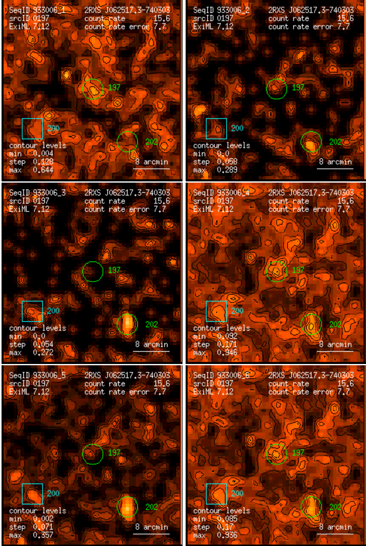
Figure 197: RASS 933006: detection 0197: band rate images, Gaussian filter: (1) PSPC channels 11 – 41, (2) 52 – 90, (3) 91 – 201, (4) 11 – 235, (5) 52 – 201, (6) 11 – 201. Broad band rates in counts/ks. Band rate contour levels in counts/ks/arcmin 2 .
