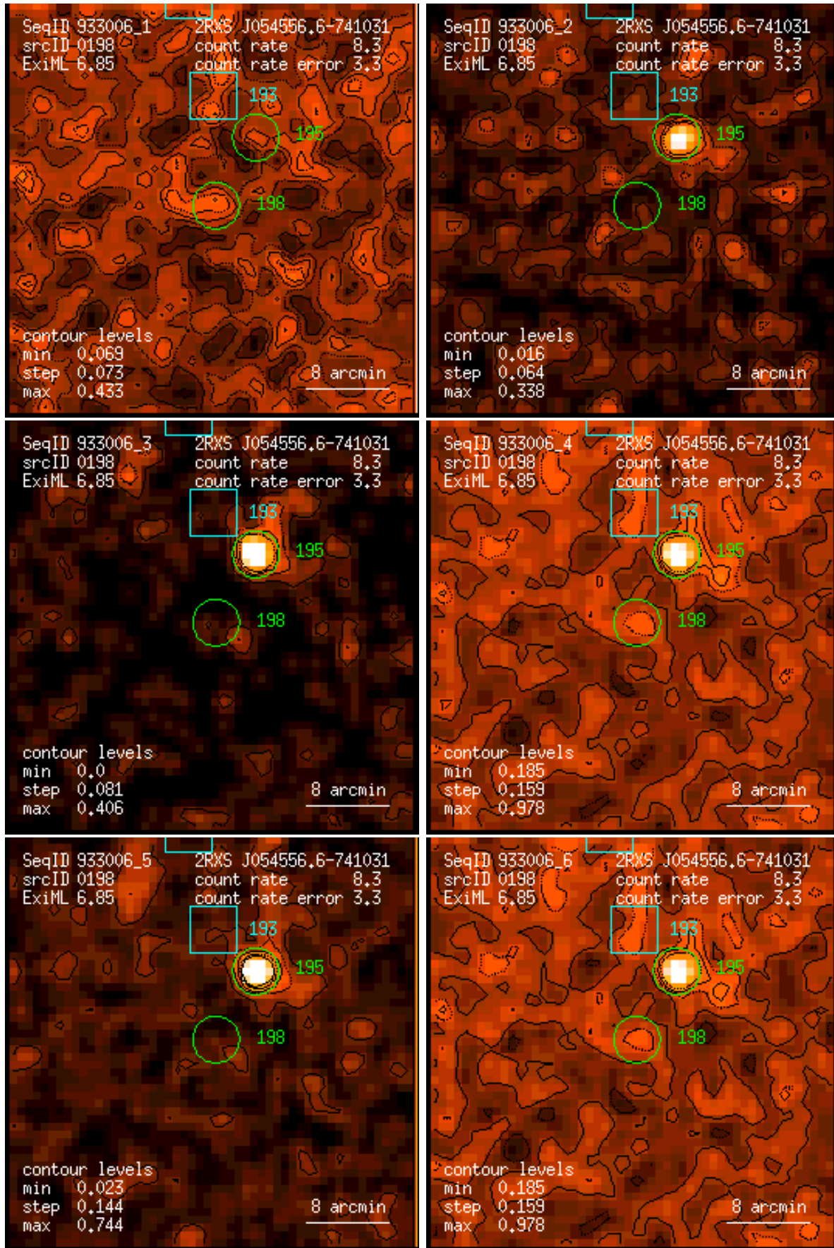
Figure 198: RASS 933006: detection 0198: band rate images, Gaussian filter: (1) PSPC channels 11 – 41, (2) 52 – 90, (3) 91 – 201, (4) 11 – 235, (5) 52 – 201, (6) 11 – 201. Broad band rates in counts/ks. Band rate contour levels in counts/ks/arcmin 2 .
