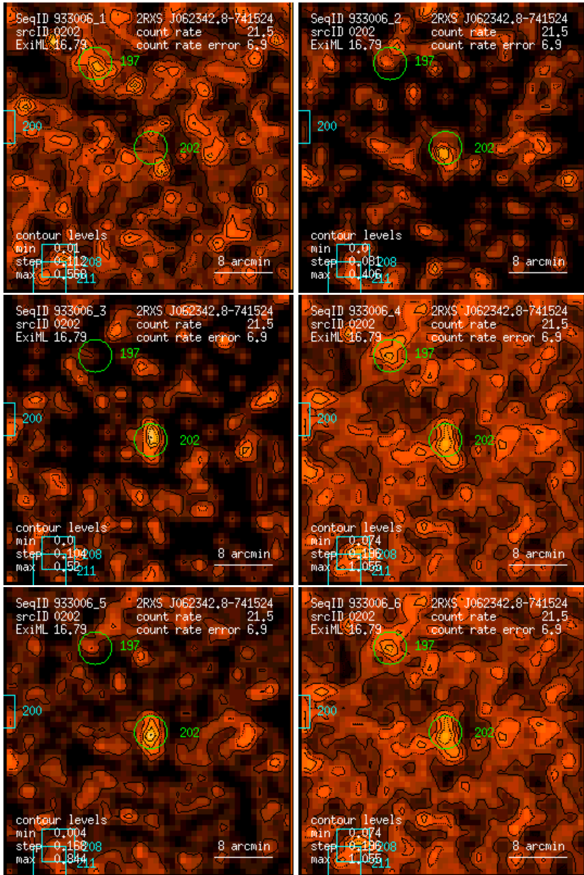
Figure 202: RASS 933006: detection 0202: band rate images, Gaussian filter: (1) PSPC channels 11 – 41, (2) 52 – 90, (3) 91 – 201, (4) 11 – 235, (5) 52 – 201, (6) 11 – 201. Broad band rates in counts/ks. Band rate contour levels in counts/ks/arcmin 2 .
