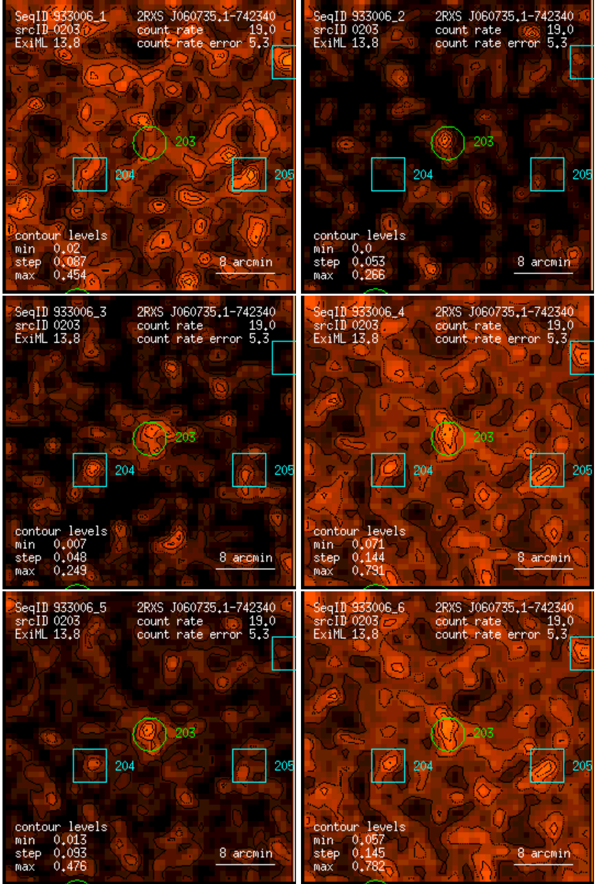
Figure 203: RASS 933006: detection 0203: band rate images, Gaussian filter: (1) PSPC channels 11 – 41, (2) 52 – 90, (3) 91 – 201, (4) 11 – 235, (5) 52 – 201, (6) 11 – 201. Broad band rates in counts/ks. Band rate contour levels in counts/ks/arcmin 2 .
