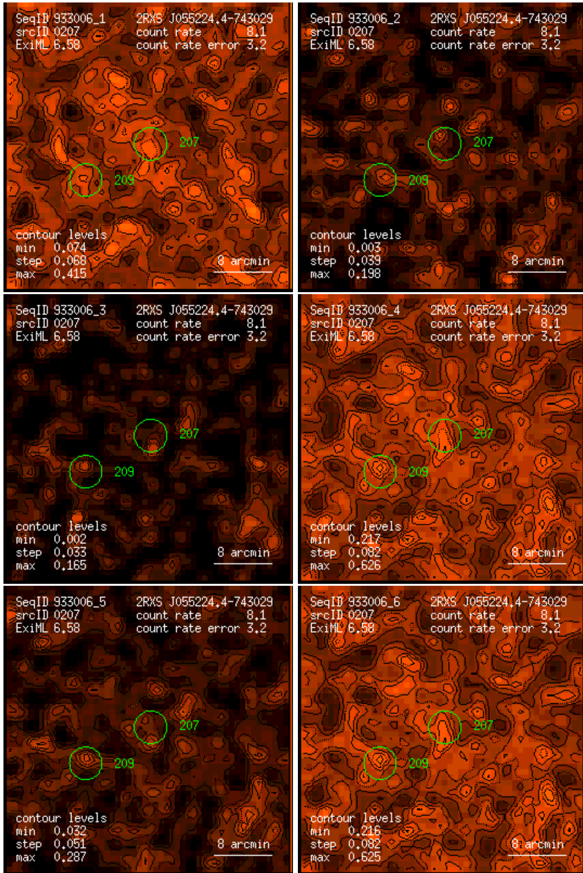
Figure 207: RASS 933006: detection 0207: band rate images, Gaussian filter: (1) PSPC channels 11 – 41, (2) 52 – 90, (3) 91 – 201, (4) 11 – 235, (5) 52 – 201, (6) 11 – 201. Broad band rates in counts/ks. Band rate contour levels in counts/ks/arcmin 2 .
