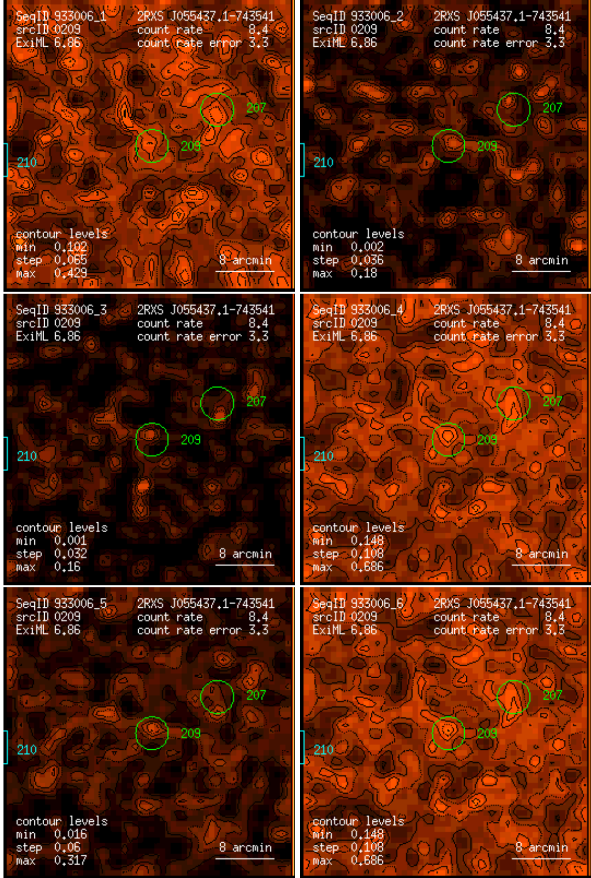
Figure 209: RASS 933006: detection 0209: band rate images, Gaussian filter: (1) PSPC channels 11 – 41, (2) 52 – 90, (3) 91 – 201, (4) 11 – 235, (5) 52 – 201, (6) 11 – 201. Broad band rates in counts/ks. Band rate contour levels in counts/ks/arcmin 2 .
