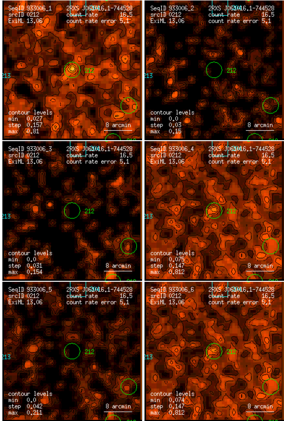
Figure 212: RASS 933006: detection 0212: band rate images, Gaussian filter: (1) PSPC channels 11 – 41, (2) 52 – 90, (3) 91 – 201, (4) 11 – 235, (5) 52 – 201, (6) 11 – 201. Broad band rates in counts/ks. Band rate contour levels in counts/ks/arcmin 2 .
