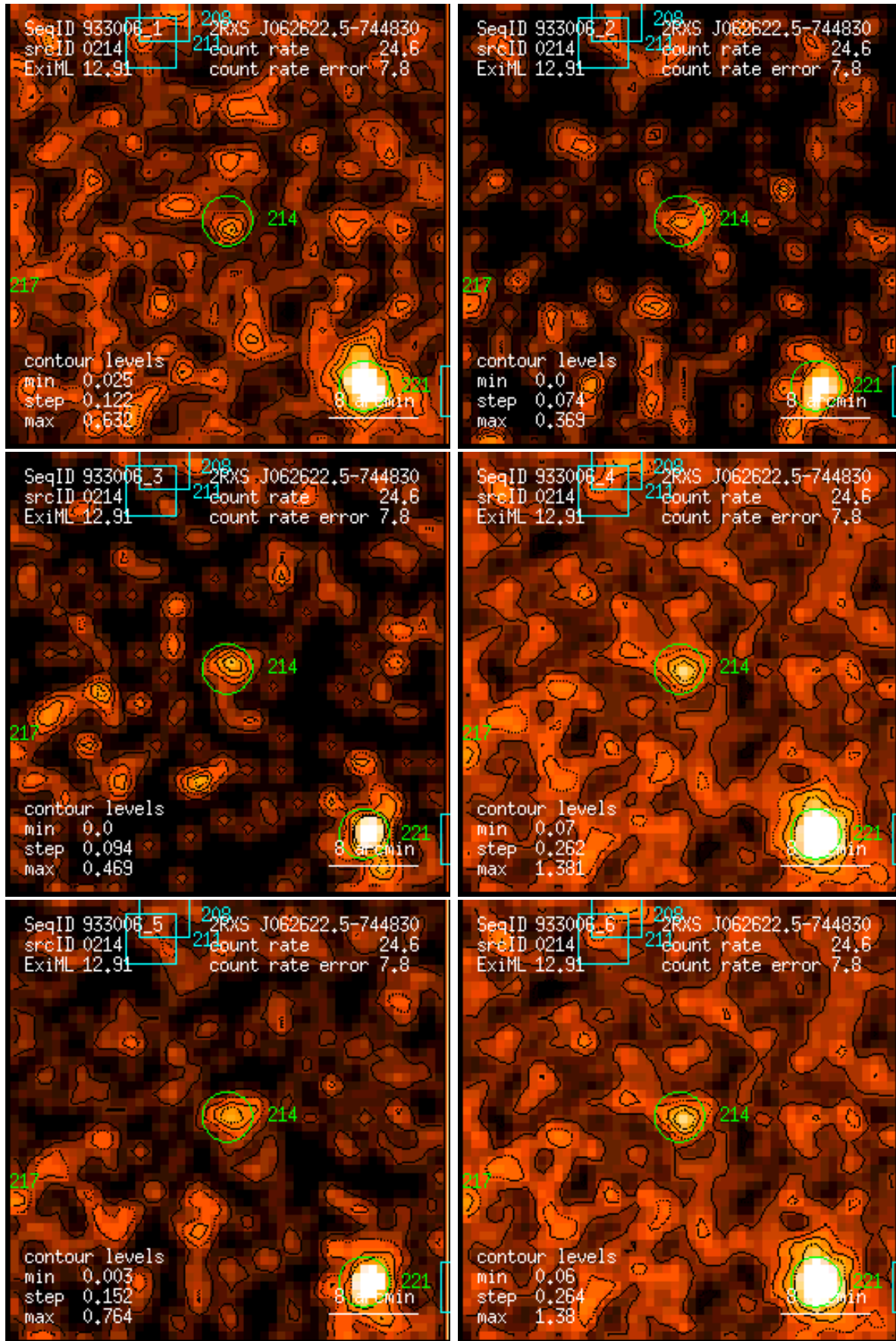
Figure 214: RASS 933006: detection 0214: band rate images, Gaussian filter: (1) PSPC channels 11 – 41, (2) 52 – 90, (3) 91 – 201, (4) 11 – 235, (5) 52 – 201, (6) 11 – 201. Broad band rates in counts/ks. Band rate contour levels in counts/ks/arcmin 2 .
