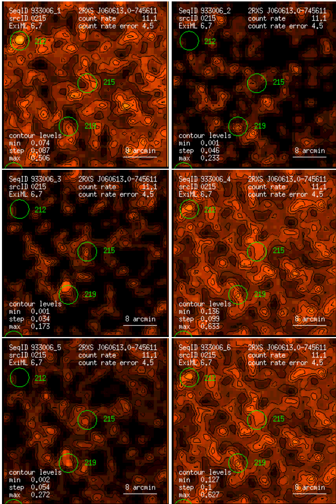
Figure 215: RASS 933006: detection 0215: band rate images, Gaussian filter: (1) PSPC channels 11 – 41, (2) 52 – 90, (3) 91 – 201, (4) 11 – 235, (5) 52 – 201, (6) 11 – 201. Broad band rates in counts/ks. Band rate contour levels in counts/ks/arcmin 2 .
