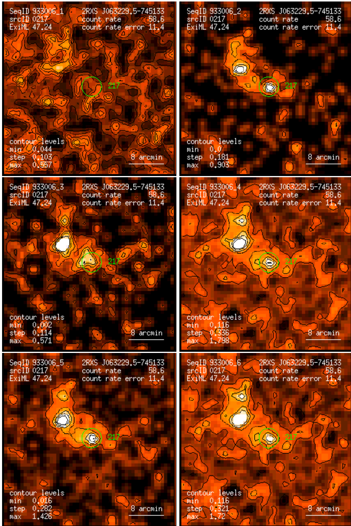
Figure 217: RASS 933006: detection 0217: band rate images, Gaussian filter: (1) PSPC channels 11 – 41, (2) 52 – 90, (3) 91 – 201, (4) 11 – 235, (5) 52 – 201, (6) 11 – 201. Broad band rates in counts/ks. Band rate contour levels in counts/ks/arcmin 2 .
