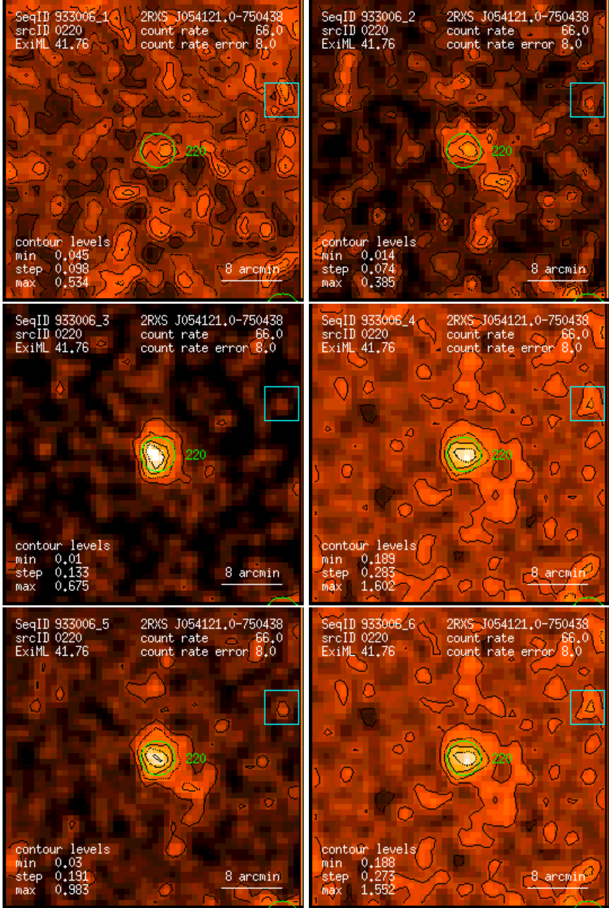
Figure 220: RASS 933006: detection 0220: band rate images, Gaussian filter: (1) PSPC channels 11 – 41, (2) 52 – 90, (3) 91 – 201, (4) 11 – 235, (5) 52 – 201, (6) 11 – 201. Broad band rates in counts/ks. Band rate contour levels in counts/ks/arcmin 2 .
