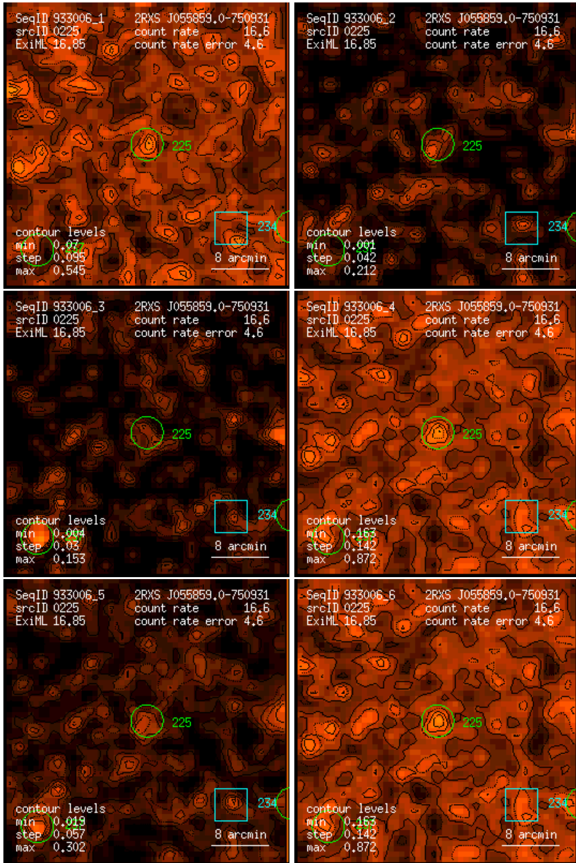
Figure 225: RASS 933006: detection 0225: band rate images, Gaussian filter: (1) PSPC channels 11 – 41, (2) 52 – 90, (3) 91 – 201, (4) 11 – 235, (5) 52 – 201, (6) 11 – 201. Broad band rates in counts/ks. Band rate contour levels in counts/ks/arcmin 2 .
