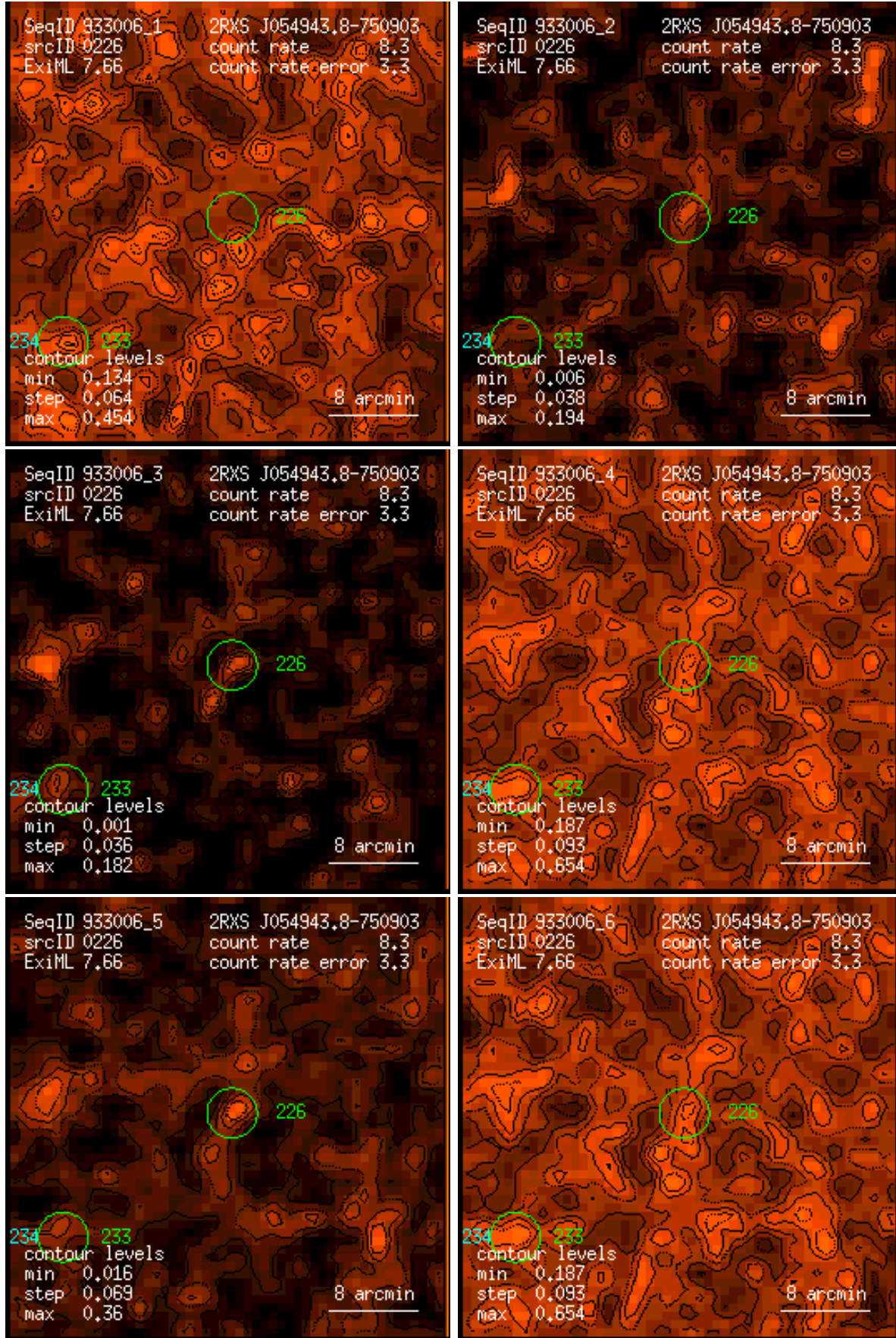
Figure 226: RASS 933006: detection 0226: band rate images, Gaussian filter: (1) PSPC channels 11 – 41, (2) 52 – 90, (3) 91 – 201, (4) 11 – 235, (5) 52 – 201, (6) 11 – 201. Broad band rates in counts/ks. Band rate contour levels in counts/ks/arcmin 2 .
