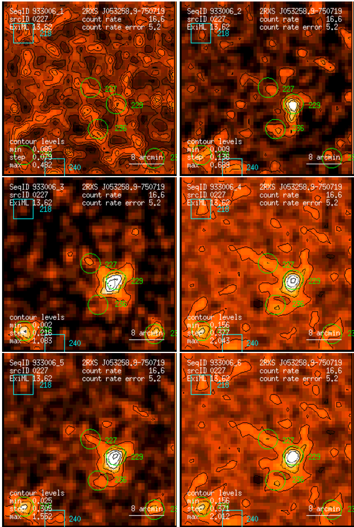
Figure 227: RASS 933006: detection 0227: band rate images, Gaussian filter: (1) PSPC channels 11 – 41, (2) 52 – 90, (3) 91 – 201, (4) 11 – 235, (5) 52 – 201, (6) 11 – 201. Broad band rates in counts/ks. Band rate contour levels in counts/ks/arcmin 2 .
