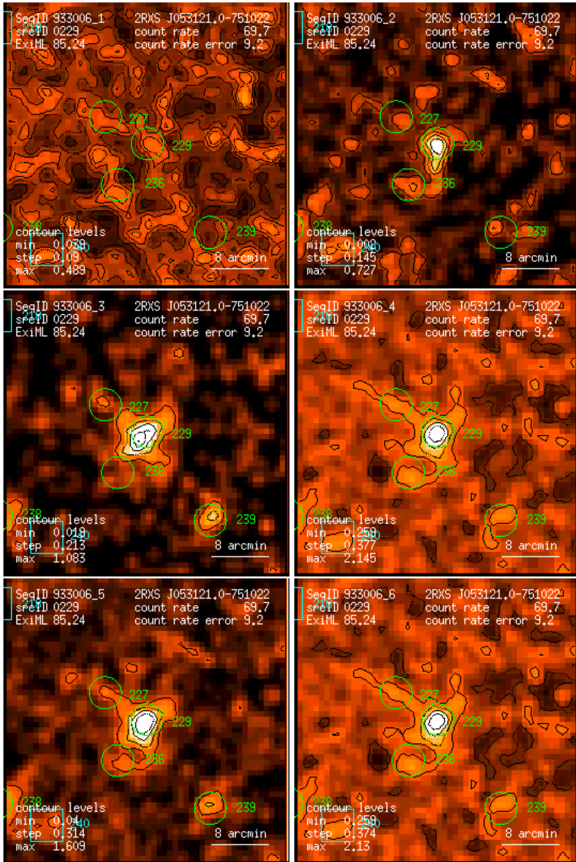
Figure 229: RASS 933006: detection 0229: band rate images, Gaussian filter: (1) PSPC channels 11 – 41, (2) 52 – 90, (3) 91 – 201, (4) 11 – 235, (5) 52 – 201, (6) 11 – 201. Broad band rates in counts/ks. Band rate contour levels in counts/ks/arcmin 2 .
