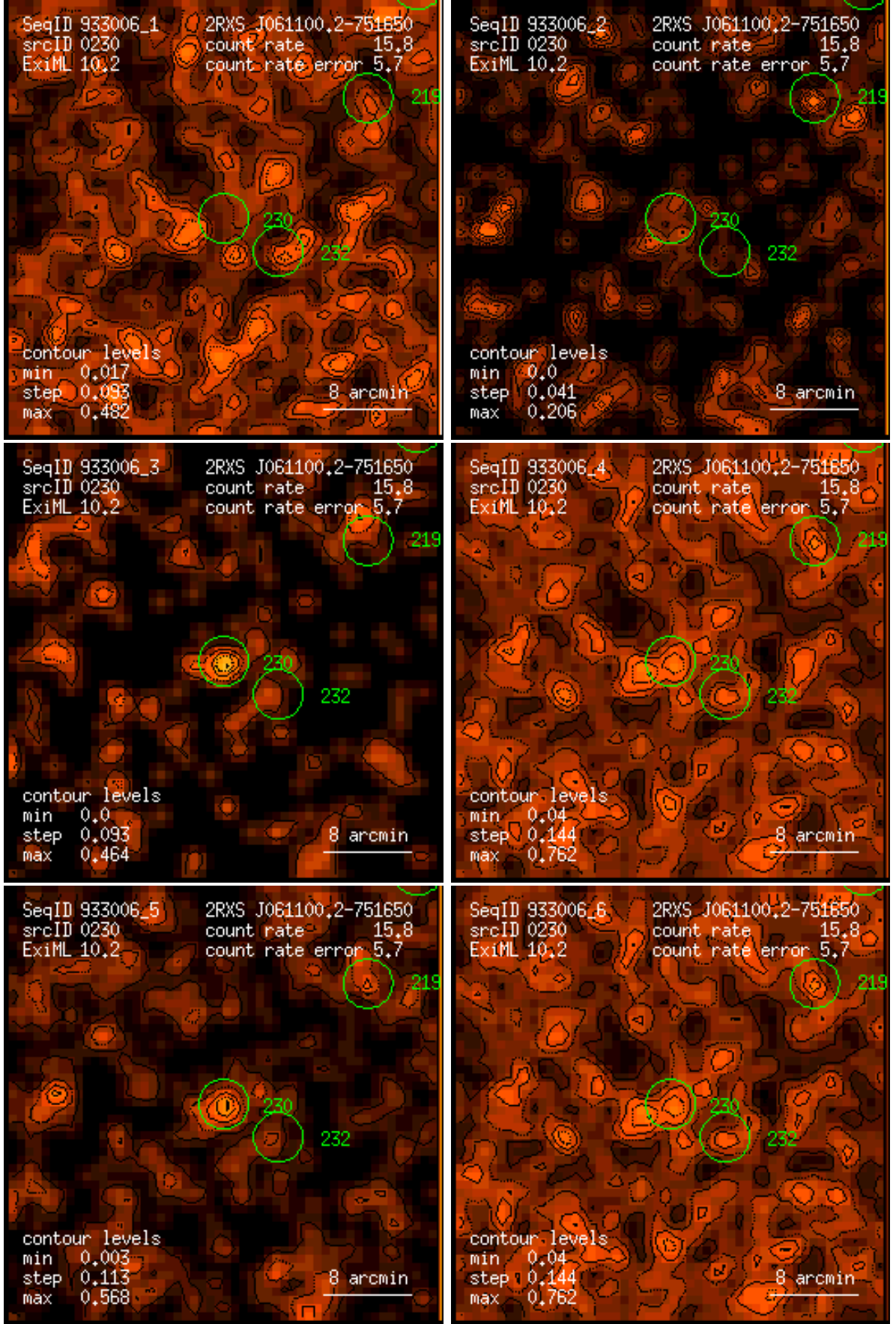
Figure 230: RASS 933006: detection 0230: band rate images, Gaussian filter: (1) PSPC channels 11 – 41, (2) 52 – 90, (3) 91 – 201, (4) 11 – 235, (5) 52 – 201, (6) 11 – 201. Broad band rates in counts/ks. Band rate contour levels in counts/ks/arcmin 2 .
