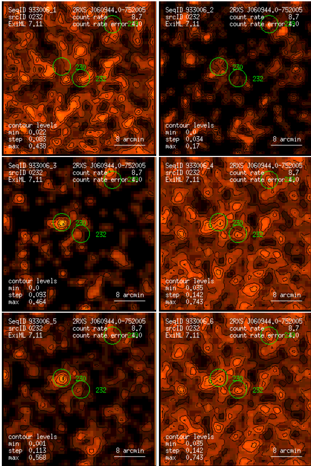
Figure 232: RASS 933006: detection 0232: band rate images, Gaussian filter: (1) PSPC channels 11 – 41, (2) 52 – 90, (3) 91 – 201, (4) 11 – 235, (5) 52 – 201, (6) 11 – 201. Broad band rates in counts/ks. Band rate contour levels in counts/ks/arcmin 2 .
