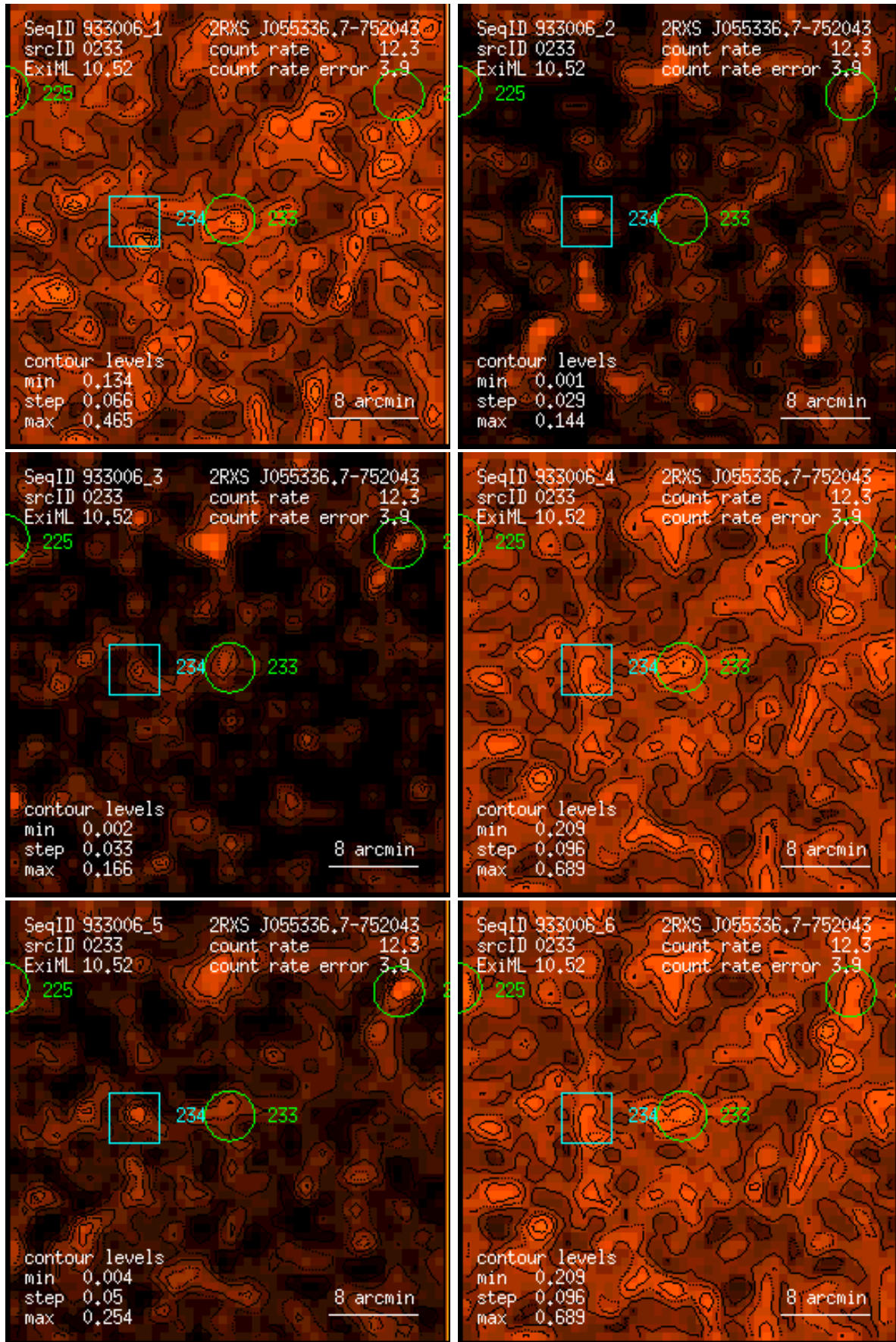
Figure 233: RASS 933006: detection 0233: band rate images, Gaussian filter: (1) PSPC channels 11 – 41, (2) 52 – 90, (3) 91 – 201, (4) 11 – 235, (5) 52 – 201, (6) 11 – 201. Broad band rates in counts/ks. Band rate contour levels in counts/ks/arcmin 2 .
