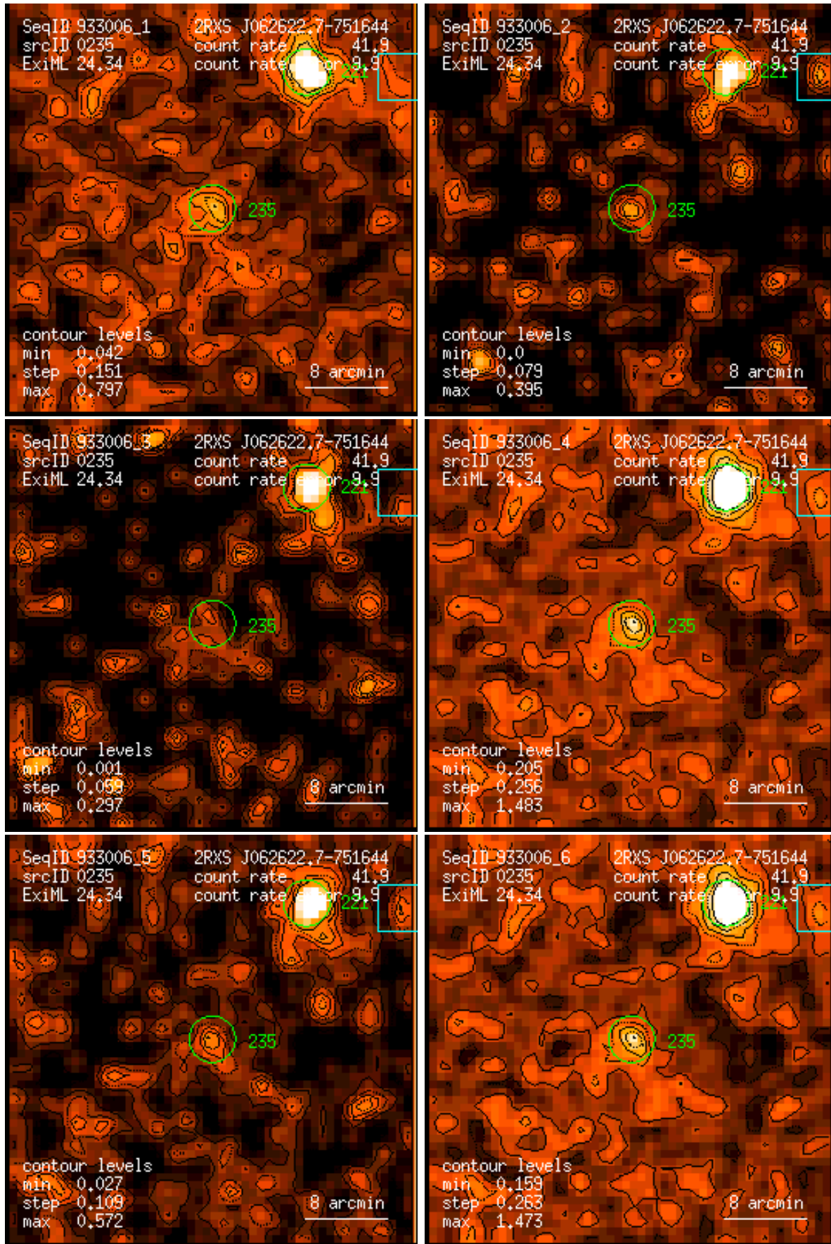
Figure 235: RASS 933006: detection 0235: band rate images, Gaussian filter: (1) PSPC channels 11 – 41, (2) 52 – 90, (3) 91 – 201, (4) 11 – 235, (5) 52 – 201, (6) 11 – 201. Broad band rates in counts/ks. Band rate contour levels in counts/ks/arcmin 2 .
