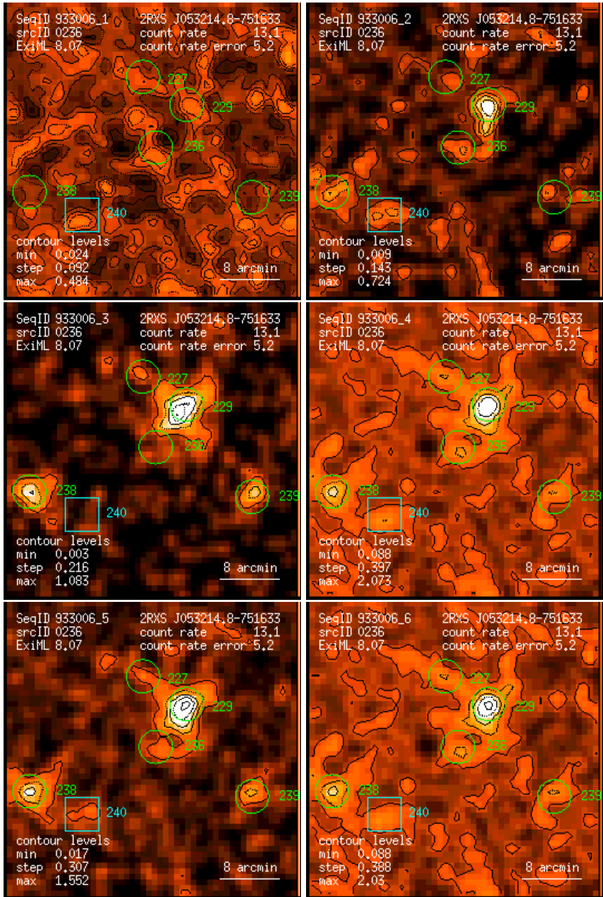
Figure 236: RASS 933006: detection 0236: band rate images, Gaussian filter: (1) PSPC channels 11 – 41, (2) 52 – 90, (3) 91 – 201, (4) 11 – 235, (5) 52 – 201, (6) 11 – 201. Broad band rates in counts/ks. Band rate contour levels in counts/ks/arcmin 2 .
