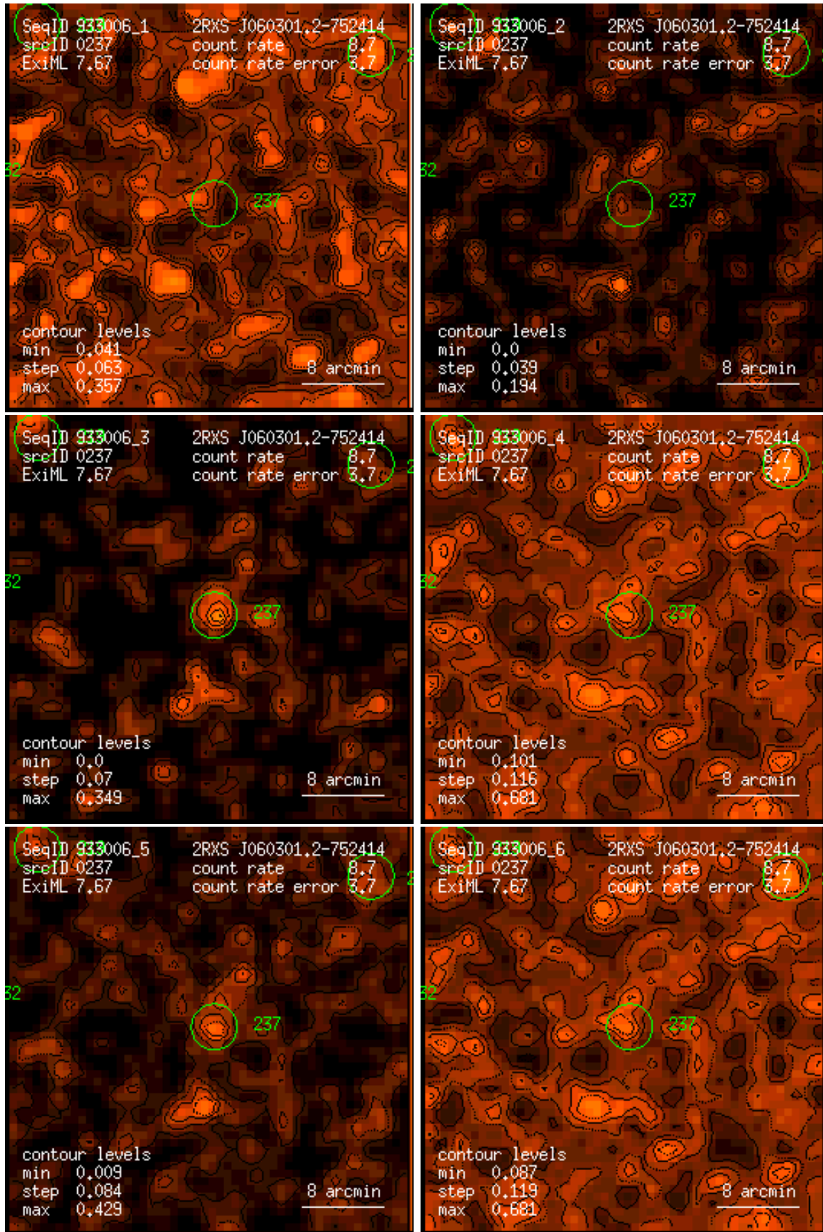
Figure 237: RASS 933006: detection 0237: band rate images, Gaussian filter: (1) PSPC channels 11 – 41, (2) 52 – 90, (3) 91 – 201, (4) 11 – 235, (5) 52 – 201, (6) 11 – 201. Broad band rates in counts/ks. Band rate contour levels in counts/ks/arcmin 2 .
