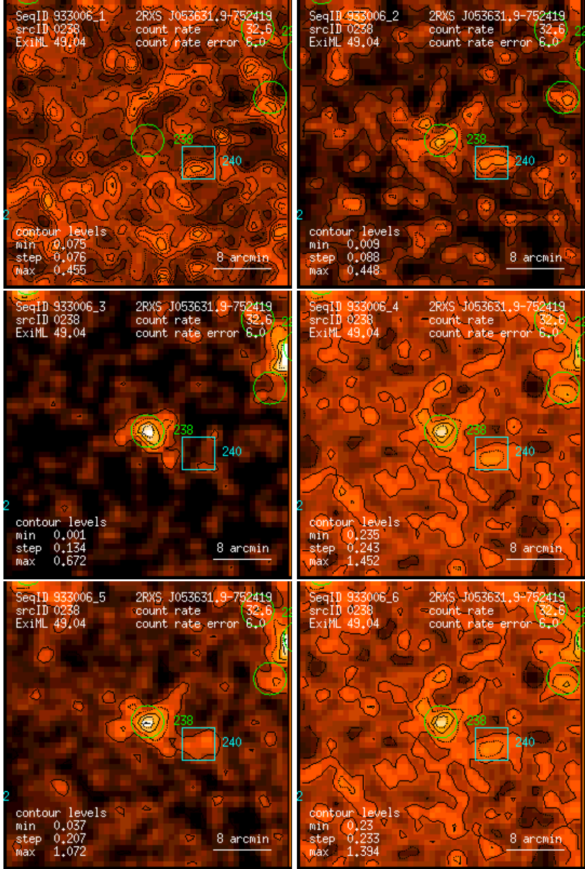
Figure 238: RASS 933006: detection 0238: band rate images, Gaussian filter: (1) PSPC channels 11 – 41, (2) 52 – 90, (3) 91 – 201, (4) 11 – 235, (5) 52 – 201, (6) 11 – 201. Broad band rates in counts/ks. Band rate contour levels in counts/ks/arcmin 2 .
