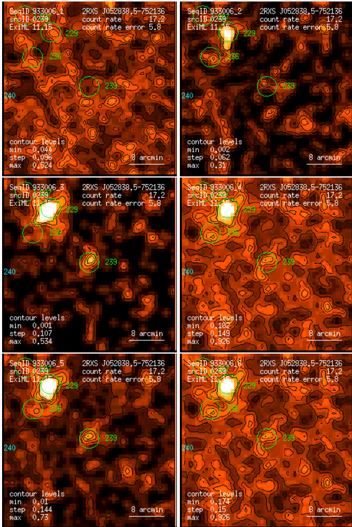
Figure 239: RASS 933006: detection 0239: band rate images, Gaussian filter: (1) PSPC channels 11 – 41, (2) 52 – 90, (3) 91 – 201, (4) 11 – 235, (5) 52 – 201, (6) 11 – 201. Broad band rates in counts/ks. Band rate contour levels in counts/ks/arcmin 2 .
