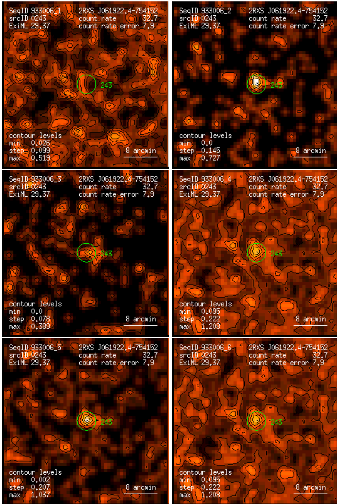
Figure 243: RASS 933006: detection 0243: band rate images, Gaussian filter: (1) PSPC channels 11 – 41, (2) 52 – 90, (3) 91 – 201, (4) 11 – 235, (5) 52 – 201, (6) 11 – 201. Broad band rates in counts/ks. Band rate contour levels in counts/ks/arcmin 2 .
