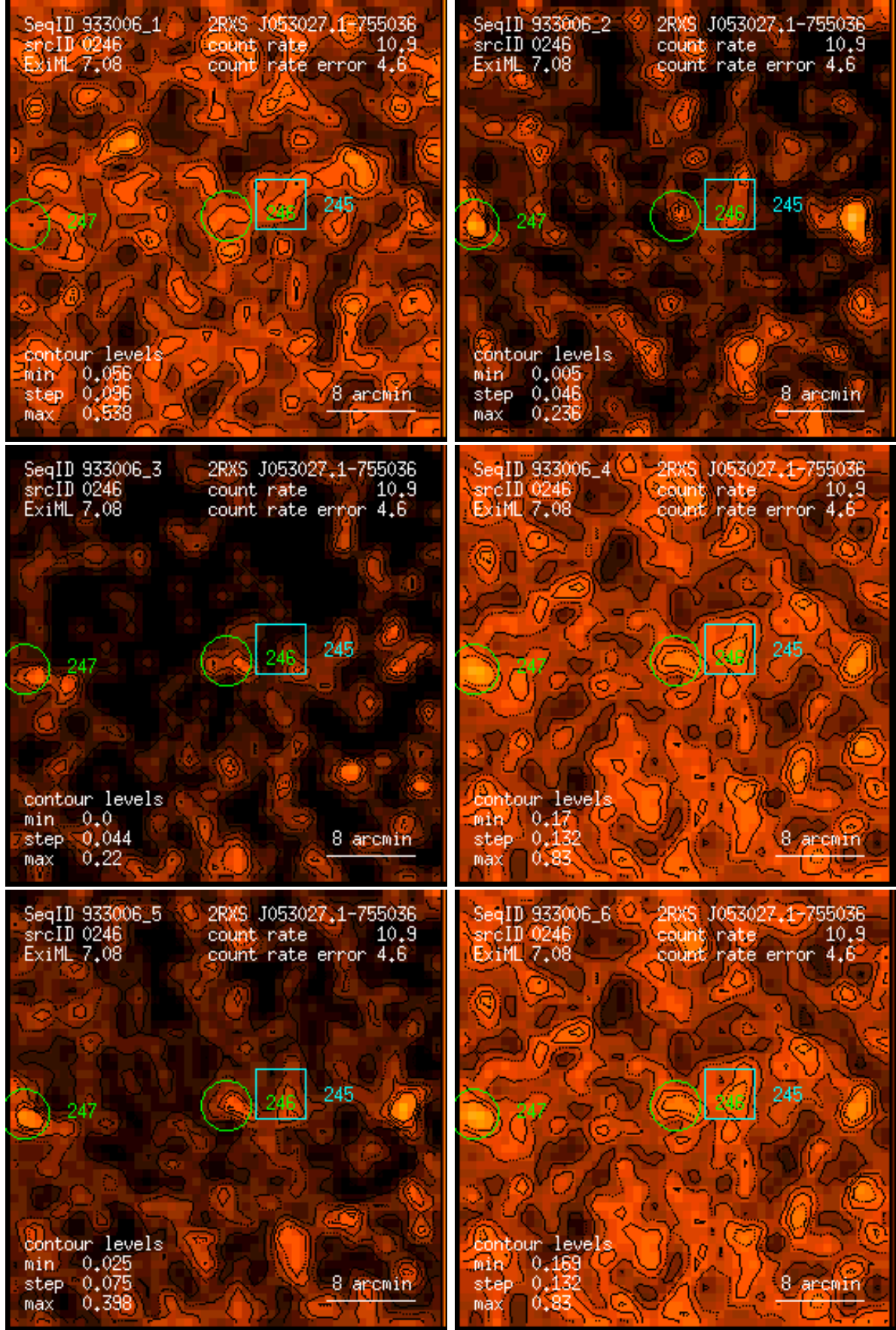
Figure 246: RASS 933006: detection 0246: band rate images, Gaussian filter: (1) PSPC channels 11 – 41, (2) 52 – 90, (3) 91 – 201, (4) 11 – 235, (5) 52 – 201, (6) 11 – 201. Broad band rates in counts/ks. Band rate contour levels in counts/ks/arcmin 2 .
