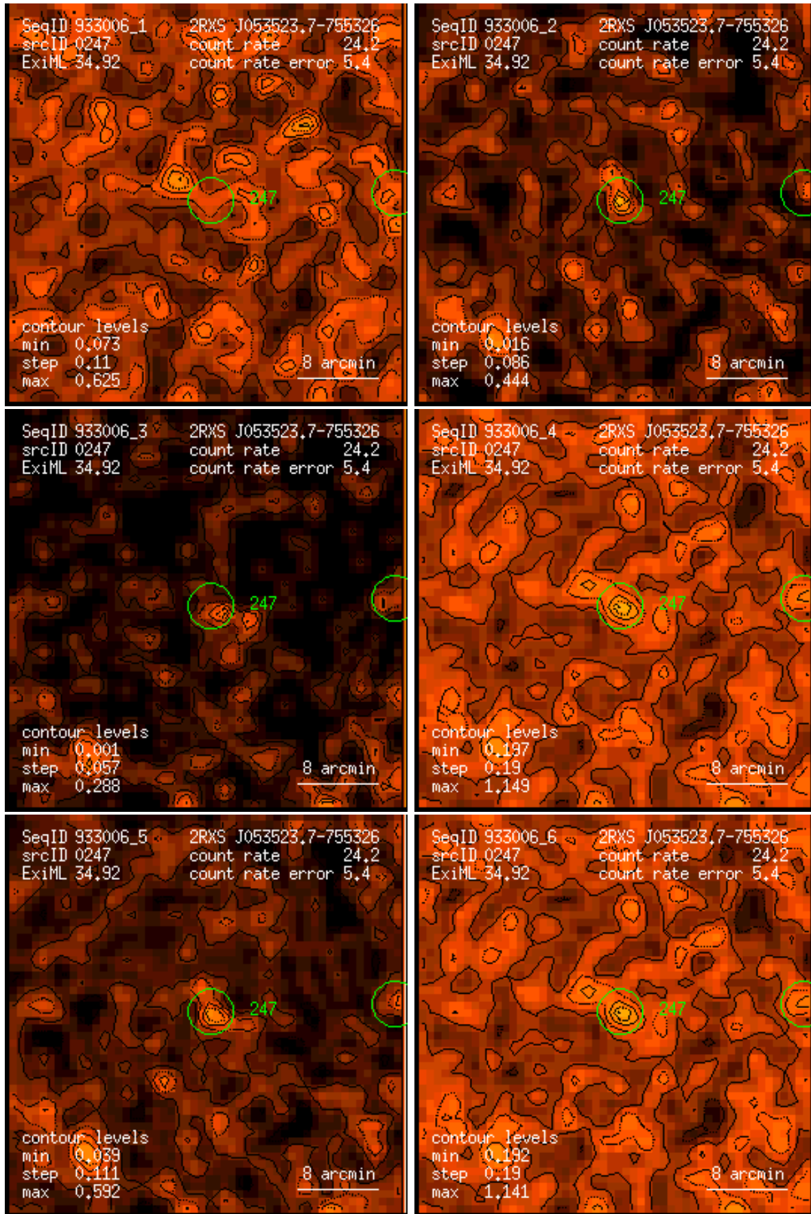
Figure 247: RASS 933006: detection 0247: band rate images, Gaussian filter: (1) PSPC channels 11 – 41, (2) 52 – 90, (3) 91 – 201, (4) 11 – 235, (5) 52 – 201, (6) 11 – 201. Broad band rates in counts/ks. Band rate contour levels in counts/ks/arcmin 2 .
