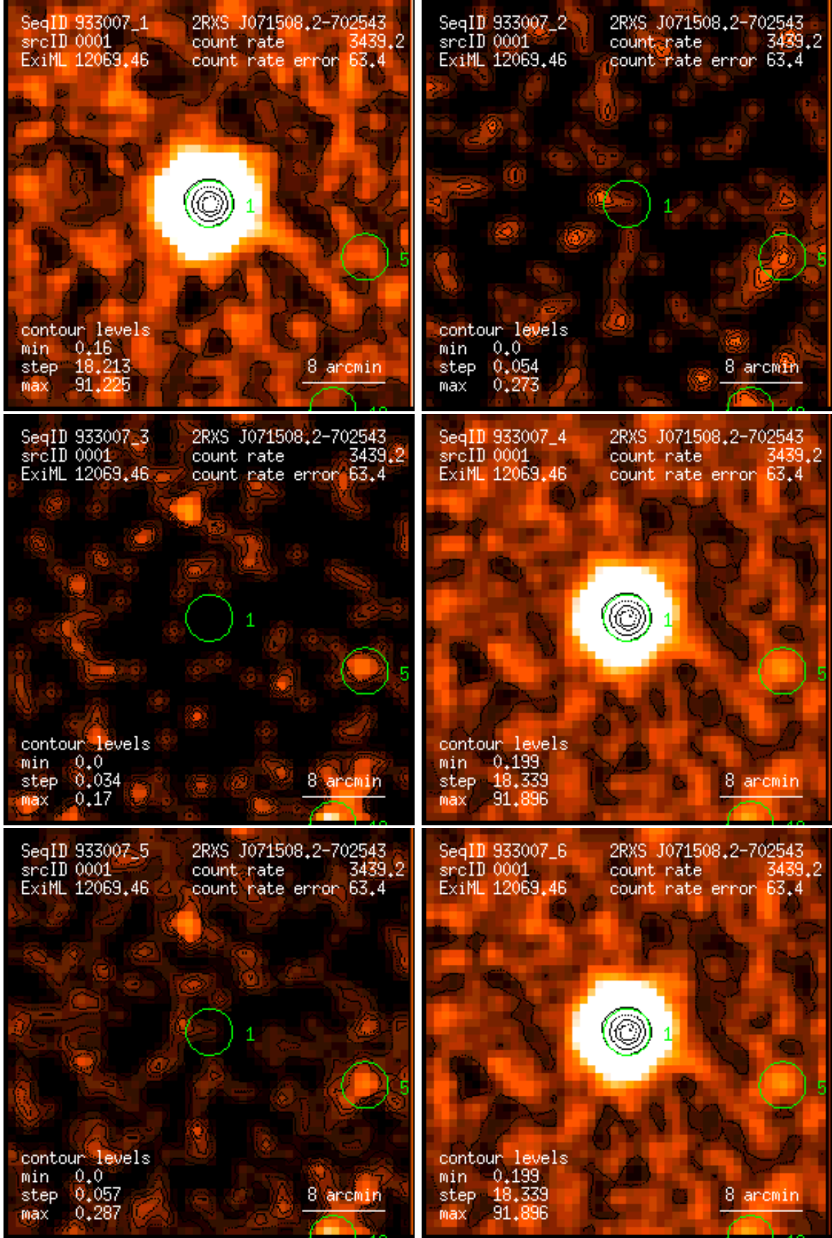
Figure 1: RASS 933007: detection 0001: band rate images, Gaussian filter: (1) PSPC channels 11 – 41, (2) 52 – 90, (3) 91 – 201, (4) 11 – 235, (5) 52 – 201, (6) 11 – 201. Broad band rates in counts/ks. Band rate contour levels in counts/ks/arcmin 2 .
