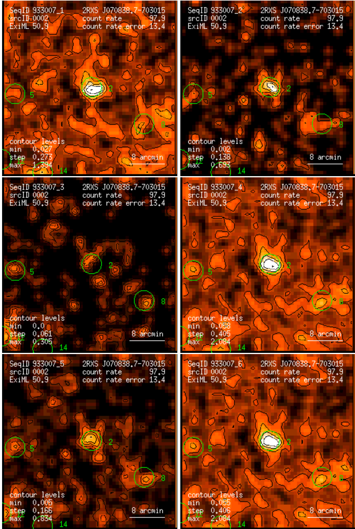
Figure 2: RASS 933007: detection 0002: band rate images, Gaussian filter: (1) PSPC channels 11 – 41, (2) 52 – 90, (3) 91 – 201, (4) 11 – 235, (5) 52 – 201, (6) 11 – 201. Broad band rates in counts/ks. Band rate contour levels in counts/ks/arcmin 2 .
