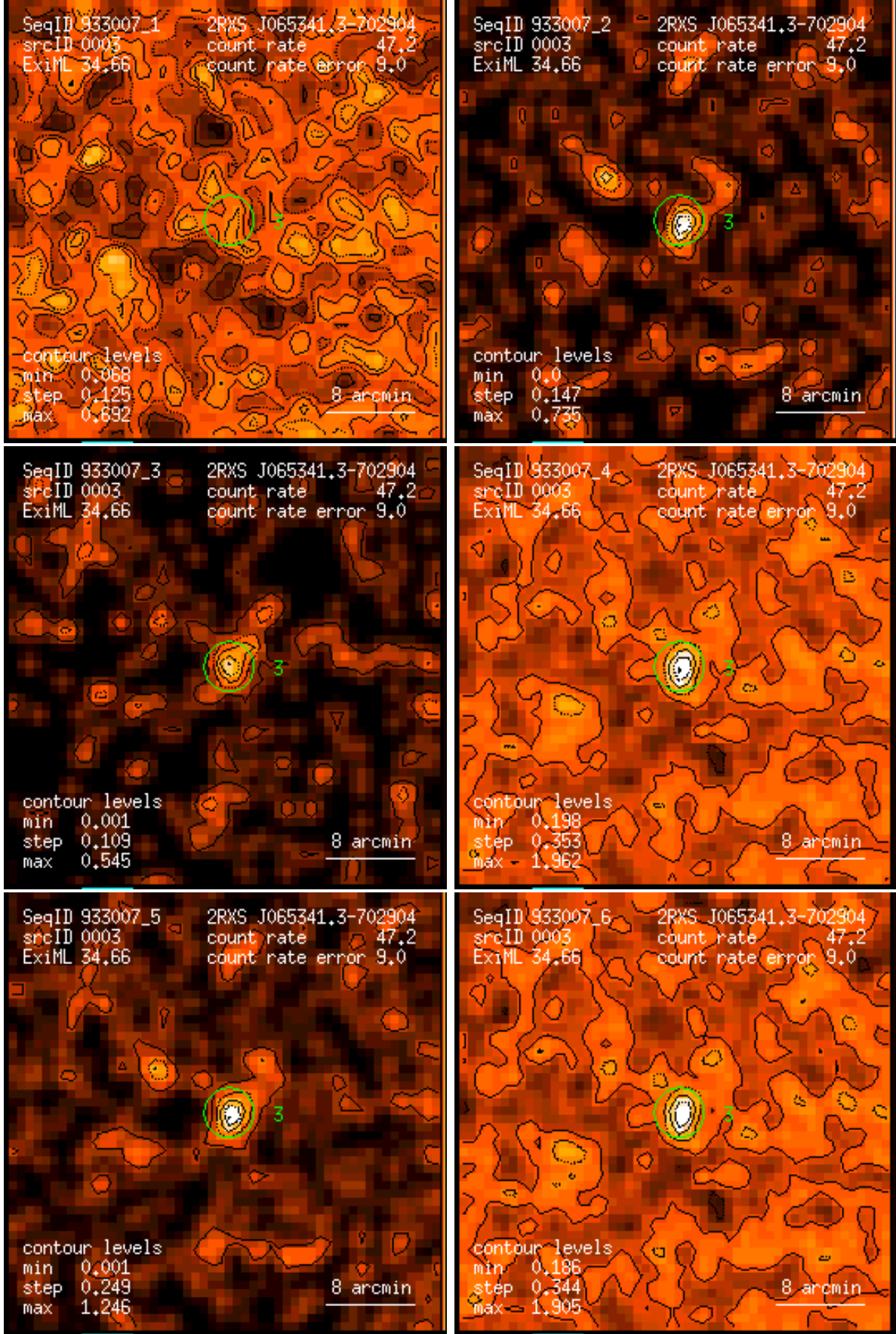
Figure 3: RASS 933007: detection 0003: band rate images, Gaussian filter: (1) PSPC channels 11 – 41, (2) 52 – 90, (3) 91 – 201, (4) 11 – 235, (5) 52 – 201, (6) 11 – 201. Broad band rates in counts/ks. Band rate contour levels in counts/ks/arcmin 2 .
