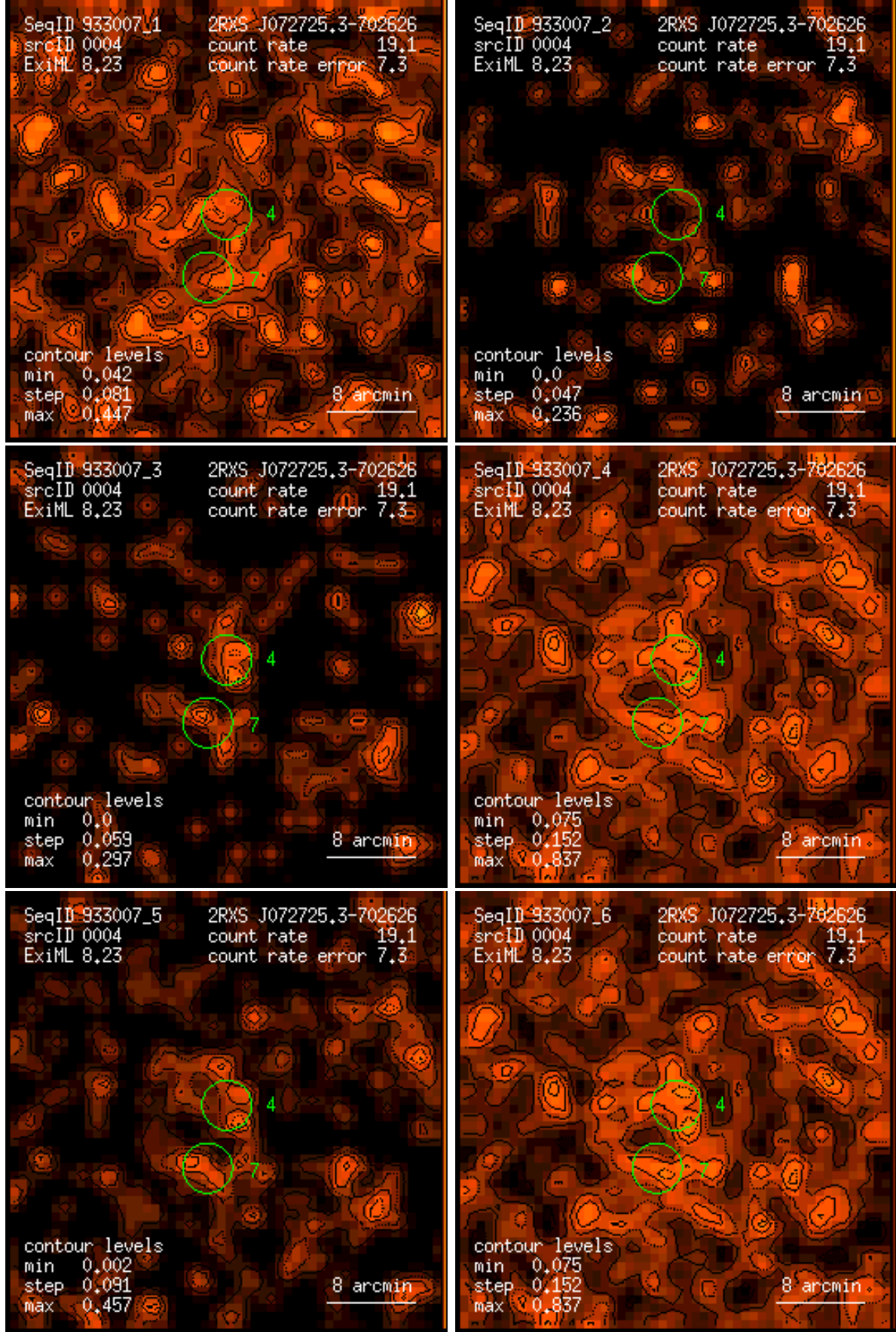
Figure 4: RASS 933007: detection 0004: band rate images, Gaussian filter: (1) PSPC channels 11 – 41, (2) 52 – 90, (3) 91 – 201, (4) 11 – 235, (5) 52 – 201, (6) 11 – 201. Broad band rates in counts/ks. Band rate contour levels in counts/ks/arcmin 2 .
