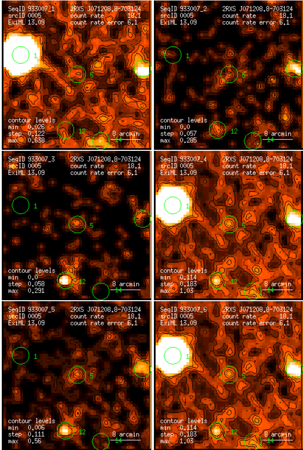
Figure 5: RASS 933007: detection 0005: band rate images, Gaussian filter: (1) PSPC channels 11 – 41, (2) 52 – 90, (3) 91 – 201, (4) 11 – 235, (5) 52 – 201, (6) 11 – 201. Broad band rates in counts/ks. Band rate contour levels in counts/ks/arcmin 2 .
