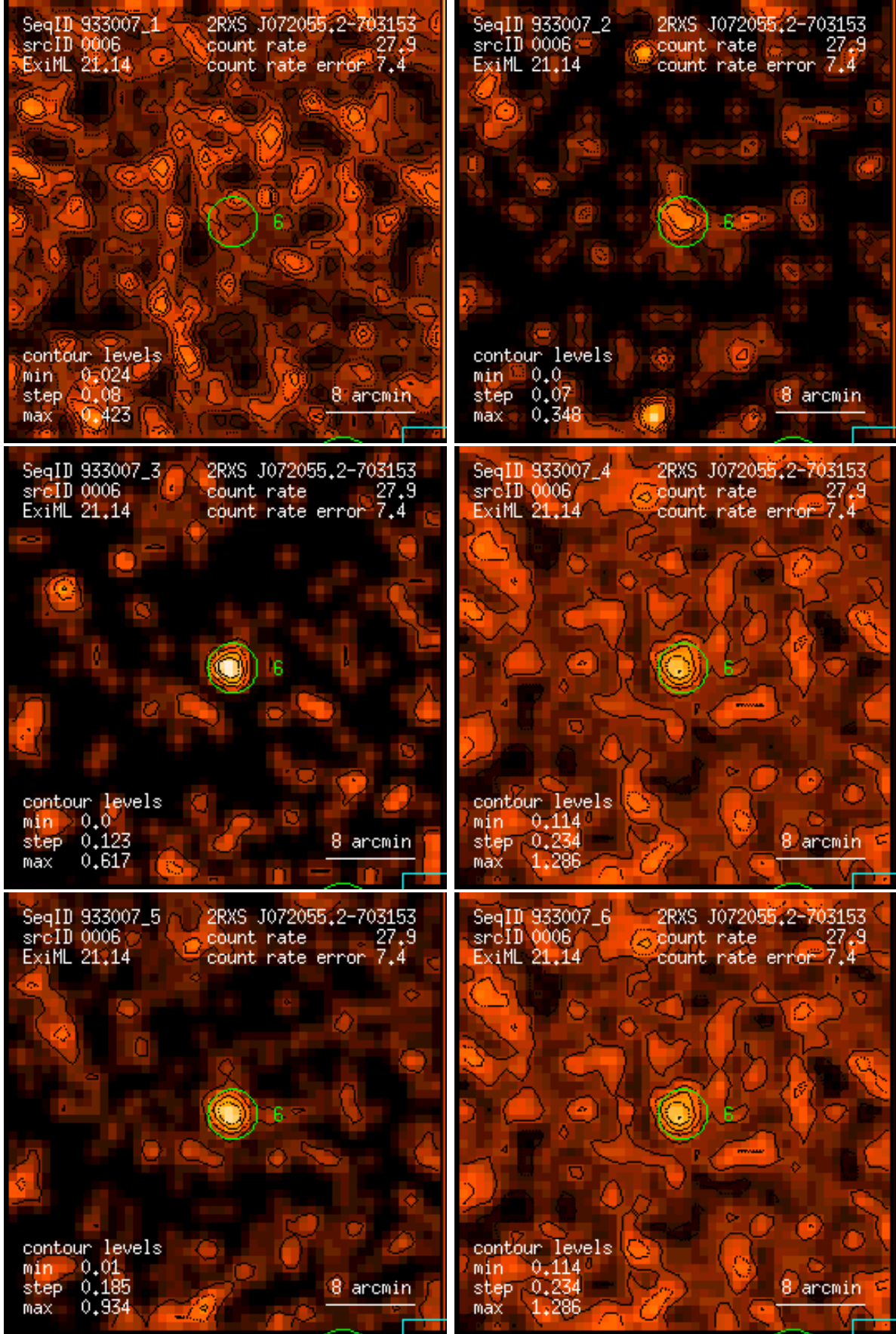
Figure 6: RASS 933007: detection 0006: band rate images, Gaussian filter: (1) PSPC channels 11 – 41, (2) 52 – 90, (3) 91 – 201, (4) 11 – 235, (5) 52 – 201, (6) 11 – 201. Broad band rates in counts/ks. Band rate contour levels in counts/ks/arcmin 2 .
