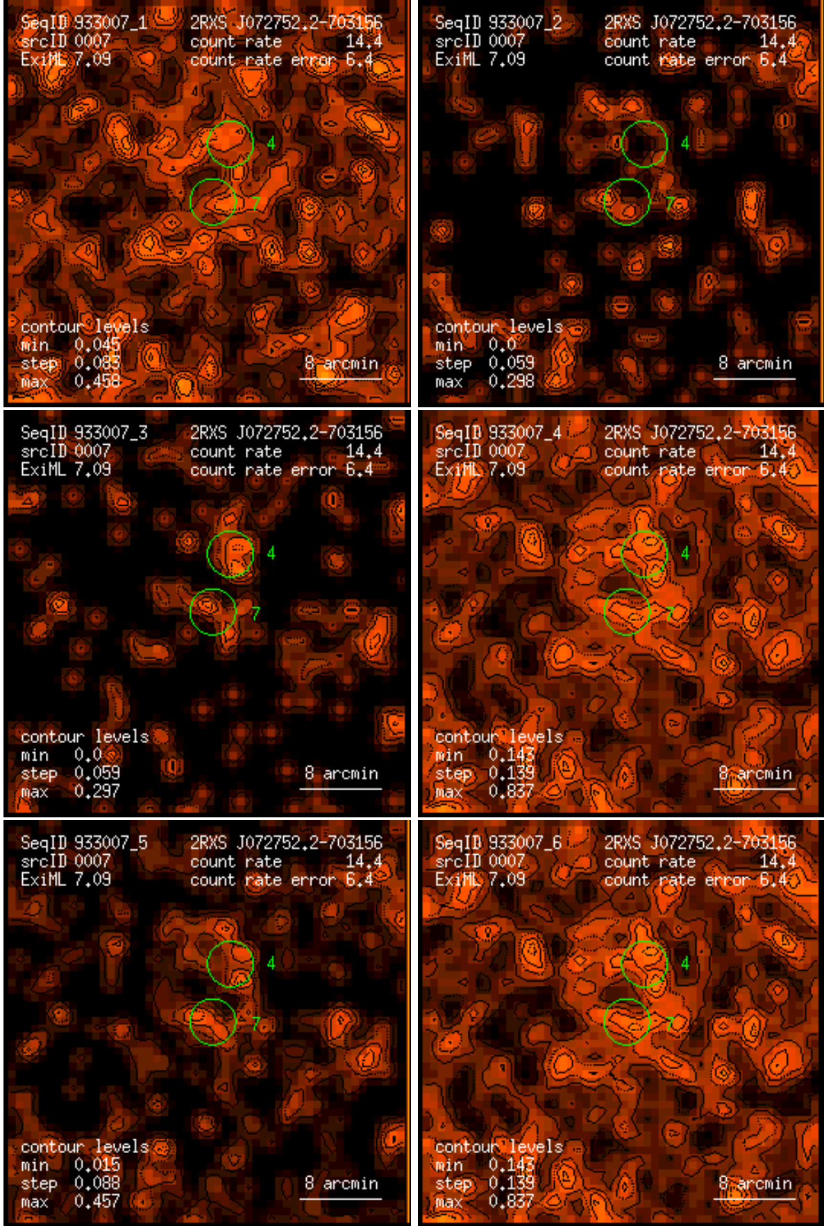
Figure 7: RASS 933007: detection 0007: band rate images, Gaussian filter: (1) PSPC channels 11 – 41, (2) 52 – 90, (3) 91 – 201, (4) 11 – 235, (5) 52 – 201, (6) 11 – 201. Broad band rates in counts/ks. Band rate contour levels in counts/ks/arcmin 2 .
