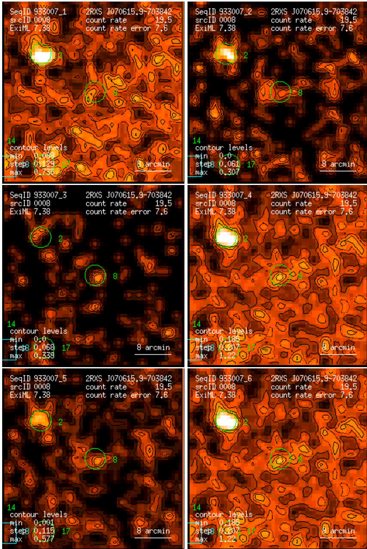
Figure 8: RASS 933007: detection 0008: band rate images, Gaussian filter: (1) PSPC channels 11 – 41, (2) 52 – 90, (3) 91 – 201, (4) 11 – 235, (5) 52 – 201, (6) 11 – 201. Broad band rates in counts/ks. Band rate contour levels in counts/ks/arcmin 2 .
