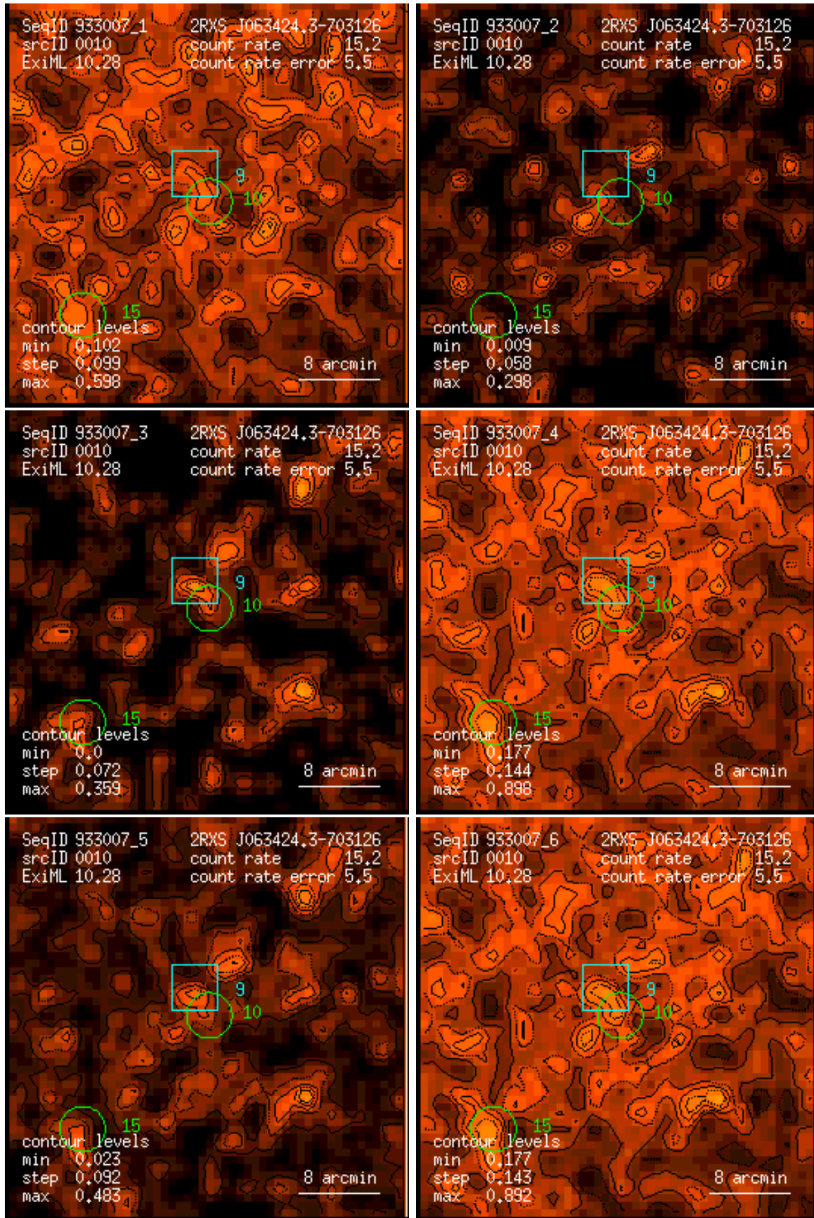
Figure 10: RASS 933007: detection 0010: band rate images, Gaussian filter: (1) PSPC channels 11 – 41, (2) 52 – 90, (3) 91 – 201, (4) 11 – 235, (5) 52 – 201, (6) 11 – 201. Broad band rates in counts/ks. Band rate contour levels in counts/ks/arcmin 2 .
