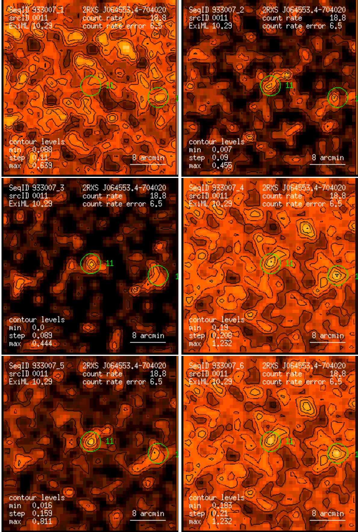
Figure 11: RASS 933007: detection 0011: band rate images, Gaussian filter: (1) PSPC channels 11 – 41, (2) 52 – 90, (3) 91 – 201, (4) 11 – 235, (5) 52 – 201, (6) 11 – 201. Broad band rates in counts/ks. Band rate contour levels in counts/ks/arcmin 2 .
