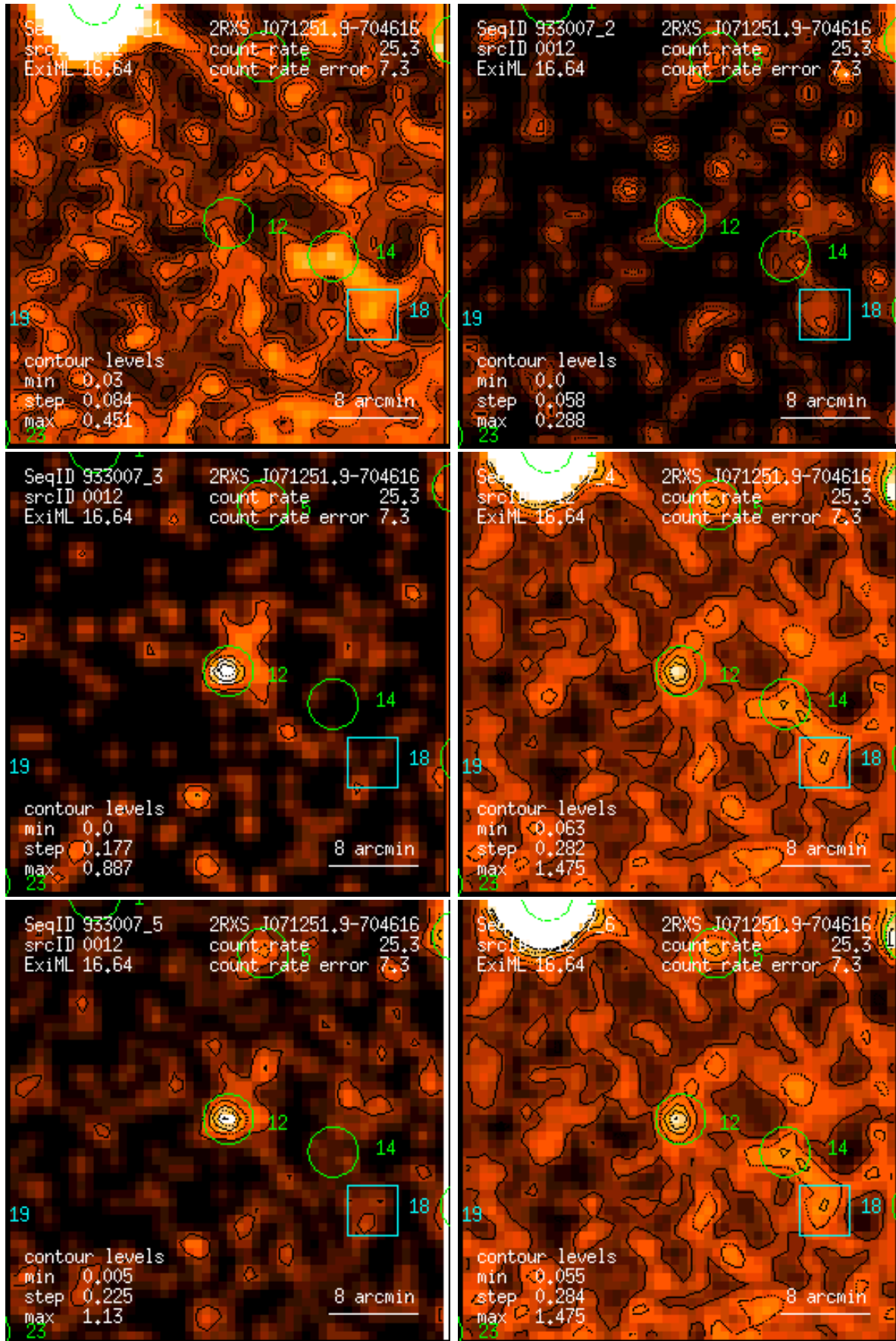
Figure 12: RASS 933007: detection 0012: band rate images, Gaussian filter: (1) PSPC channels 11 – 41, (2) 52 – 90, (3) 91 – 201, (4) 11 – 235, (5) 52 – 201, (6) 11 – 201. Broad band rates in counts/ks. Band rate contour levels in counts/ks/arcmin 2 .
