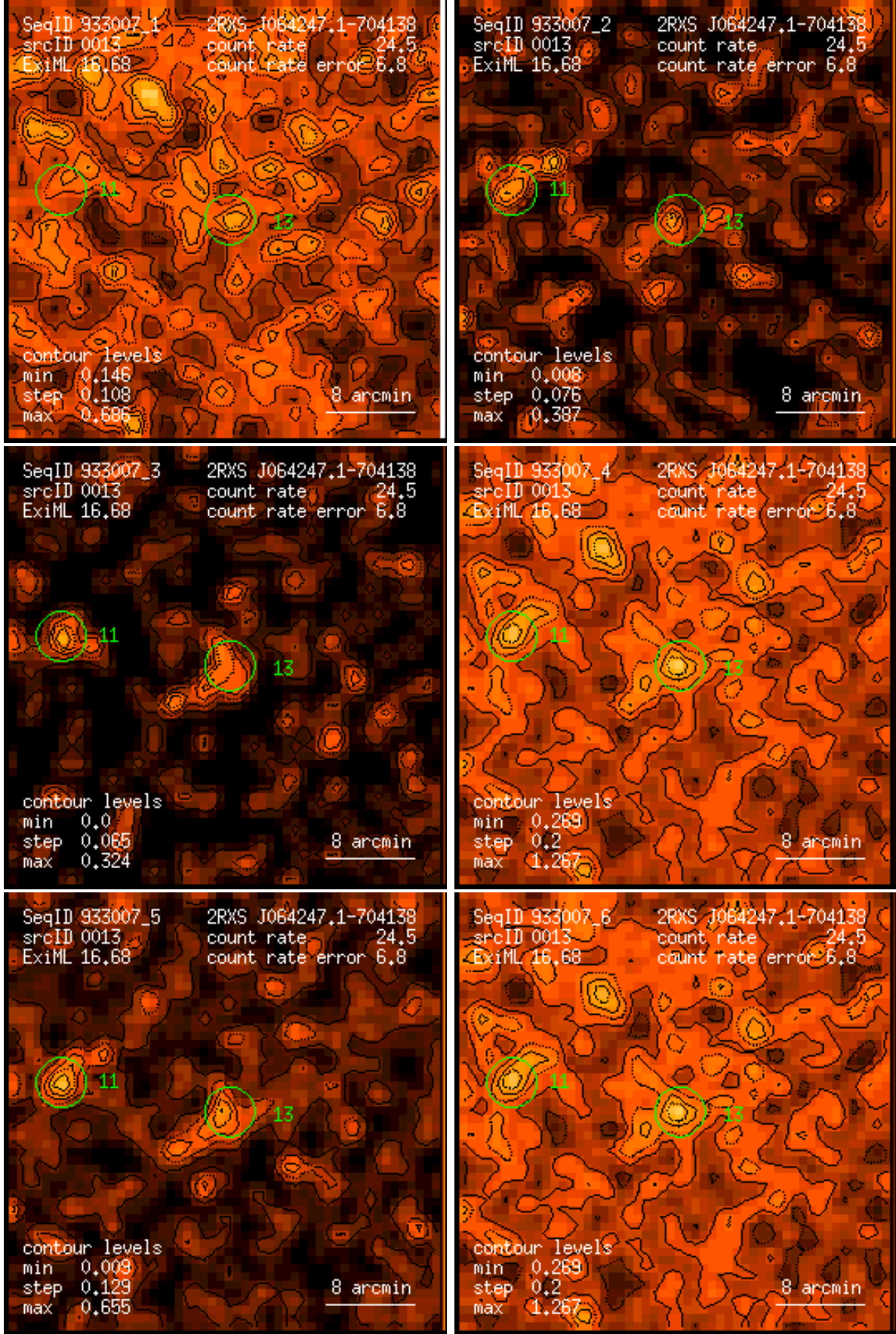
Figure 13: RASS 933007: detection 0013: band rate images, Gaussian filter: (1) PSPC channels 11 – 41, (2) 52 – 90, (3) 91 – 201, (4) 11 – 235, (5) 52 – 201, (6) 11 – 201. Broad band rates in counts/ks. Band rate contour levels in counts/ks/arcmin 2 .
