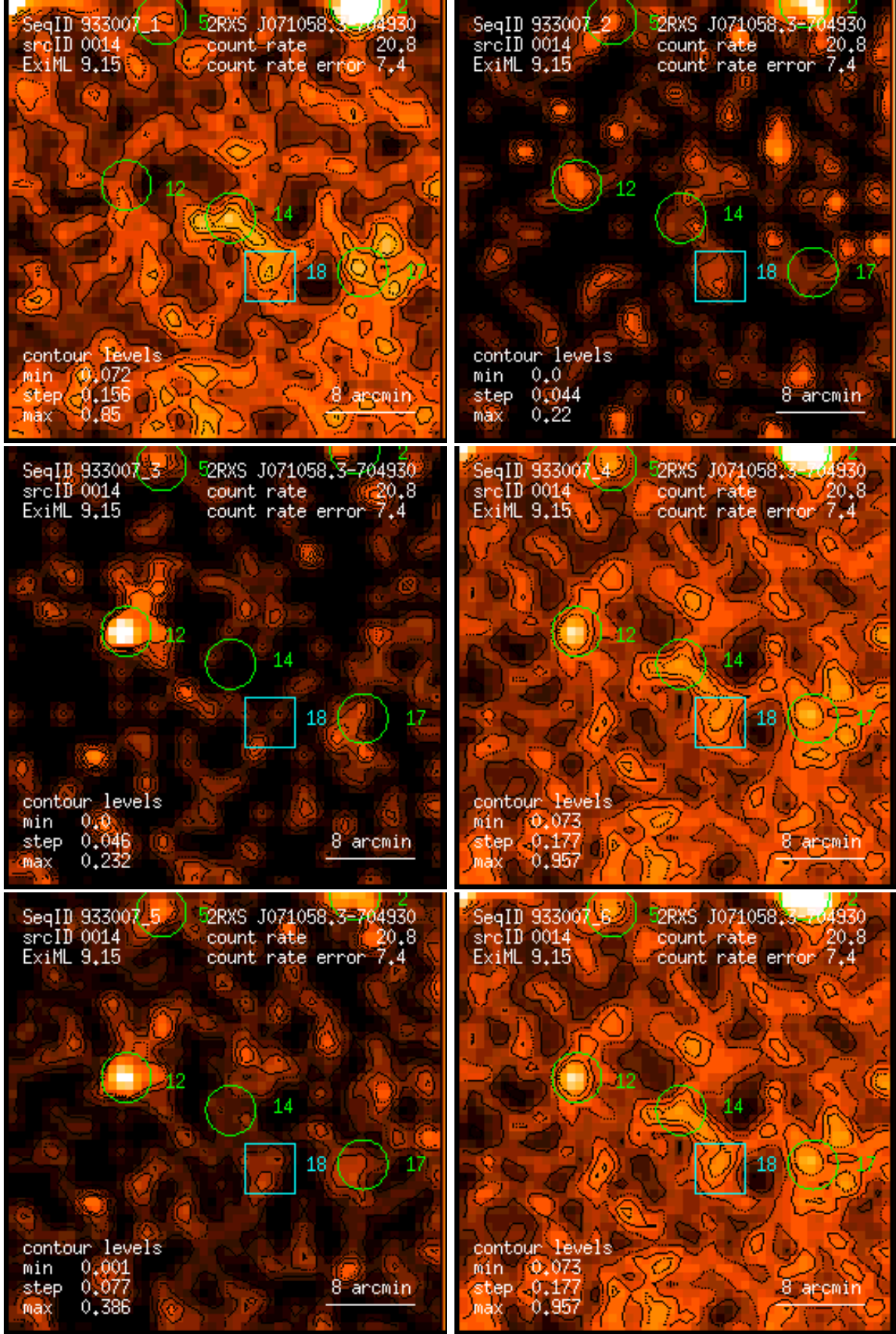
Figure 14: RASS 933007: detection 0014: band rate images, Gaussian filter: (1) PSPC channels 11 – 41, (2) 52 – 90, (3) 91 – 201, (4) 11 – 235, (5) 52 – 201, (6) 11 – 201. Broad band rates in counts/ks. Band rate contour levels in counts/ks/arcmin 2 .
