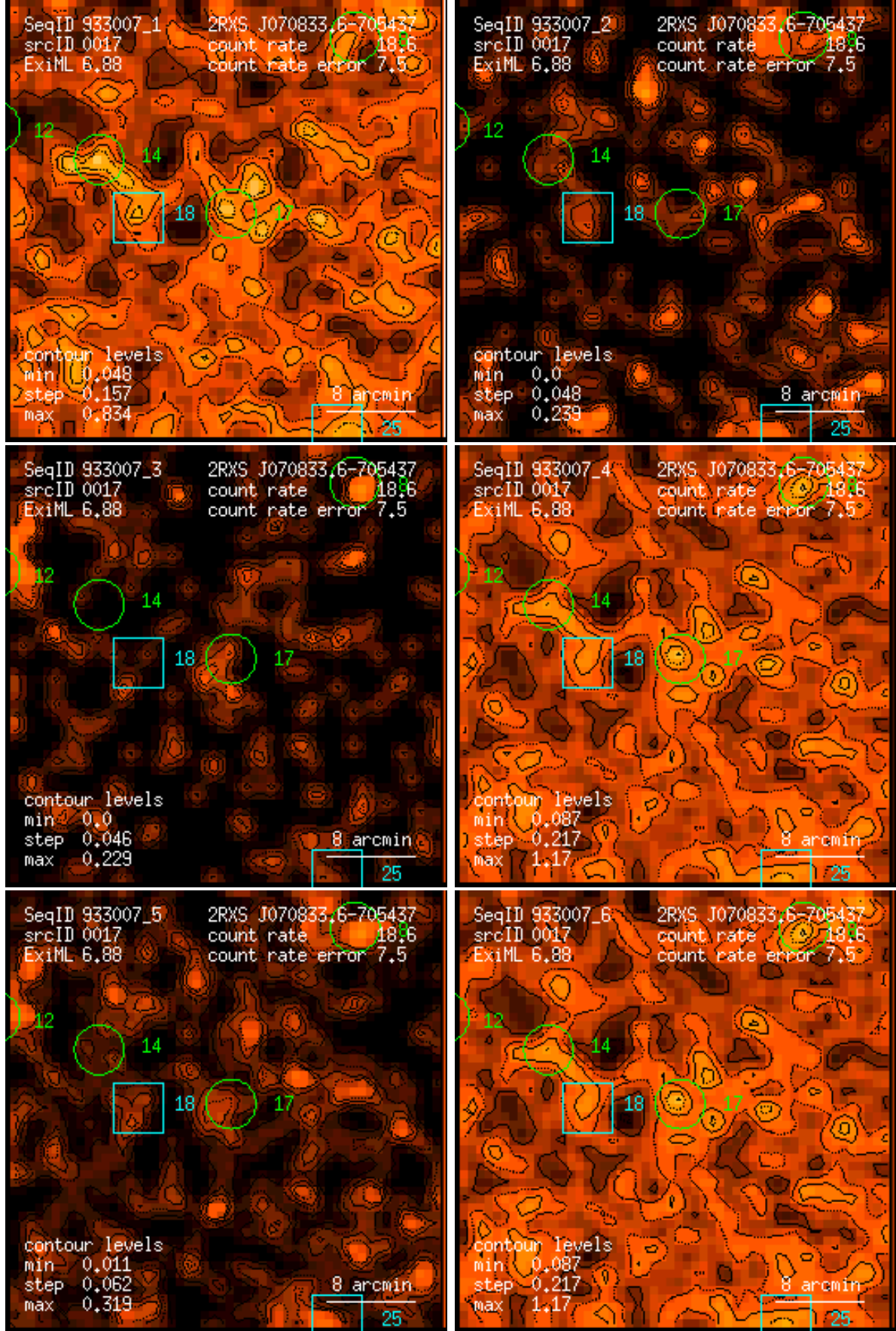
Figure 17: RASS 933007: detection 0017: band rate images, Gaussian filter: (1) PSPC channels 11 – 41, (2) 52 – 90, (3) 91 – 201, (4) 11 – 235, (5) 52 – 201, (6) 11 – 201. Broad band rates in counts/ks. Band rate contour levels in counts/ks/arcmin 2 .
