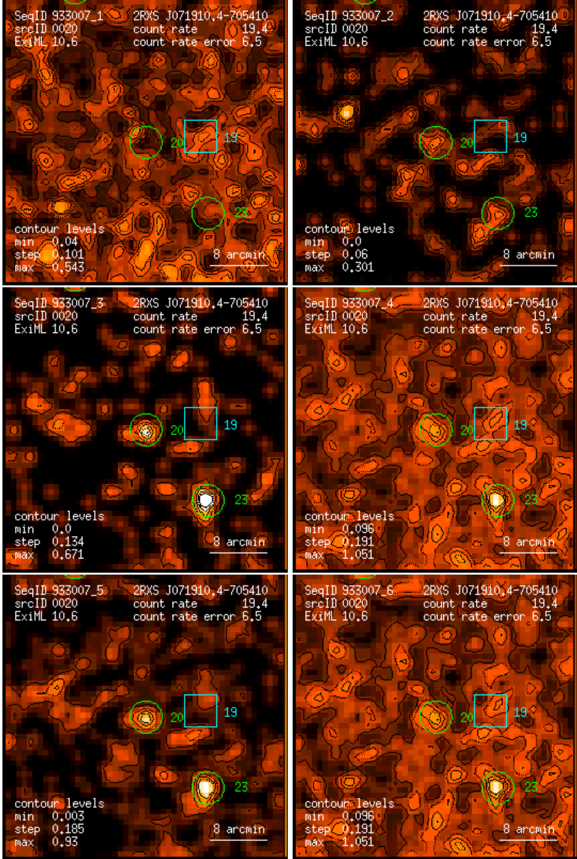
Figure 20: RASS 933007: detection 0020: band rate images, Gaussian filter: (1) PSPC channels 11 – 41, (2) 52 – 90, (3) 91 – 201, (4) 11 – 235, (5) 52 – 201, (6) 11 – 201. Broad band rates in counts/ks. Band rate contour levels in counts/ks/arcmin 2 .
