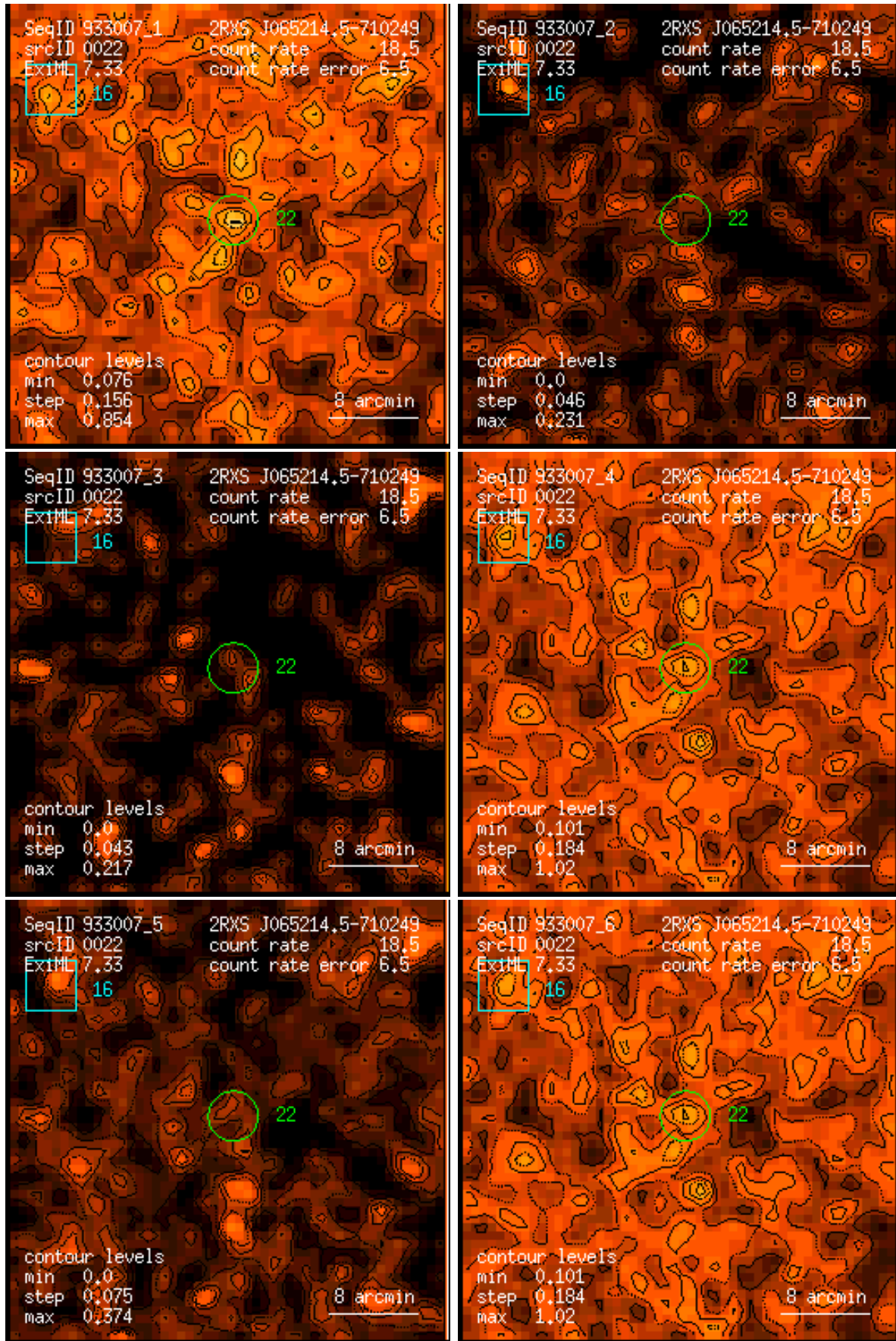
Figure 22: RASS 933007: detection 0022: band rate images, Gaussian filter: (1) PSPC channels 11 – 41, (2) 52 – 90, (3) 91 – 201, (4) 11 – 235, (5) 52 – 201, (6) 11 – 201. Broad band rates in counts/ks. Band rate contour levels in counts/ks/arcmin 2 .
