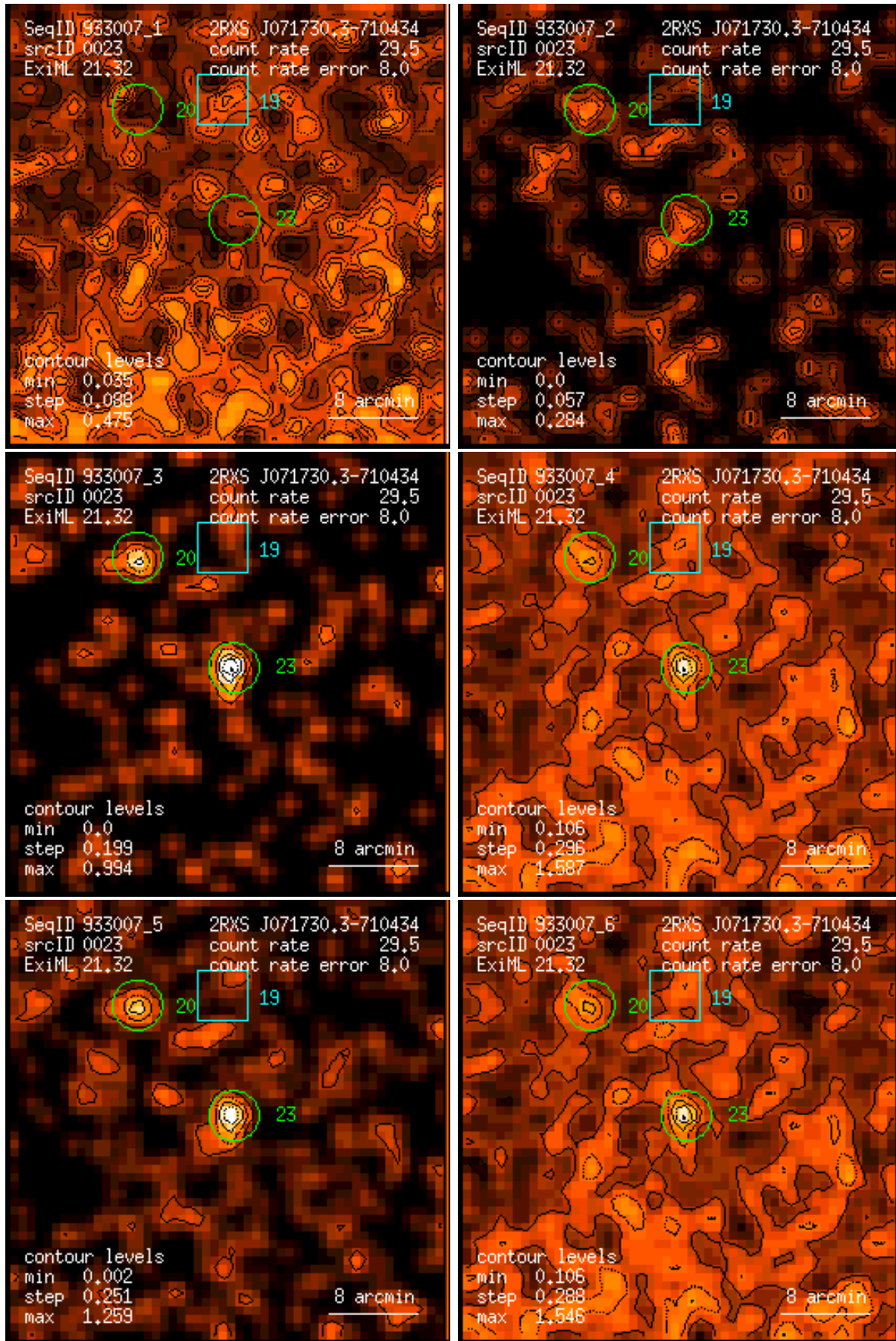
Figure 23: RASS 933007: detection 0023: band rate images, Gaussian filter: (1) PSPC channels 11 – 41, (2) 52 – 90, (3) 91 – 201, (4) 11 – 235, (5) 52 – 201, (6) 11 – 201. Broad band rates in counts/ks. Band rate contour levels in counts/ks/arcmin 2 .
