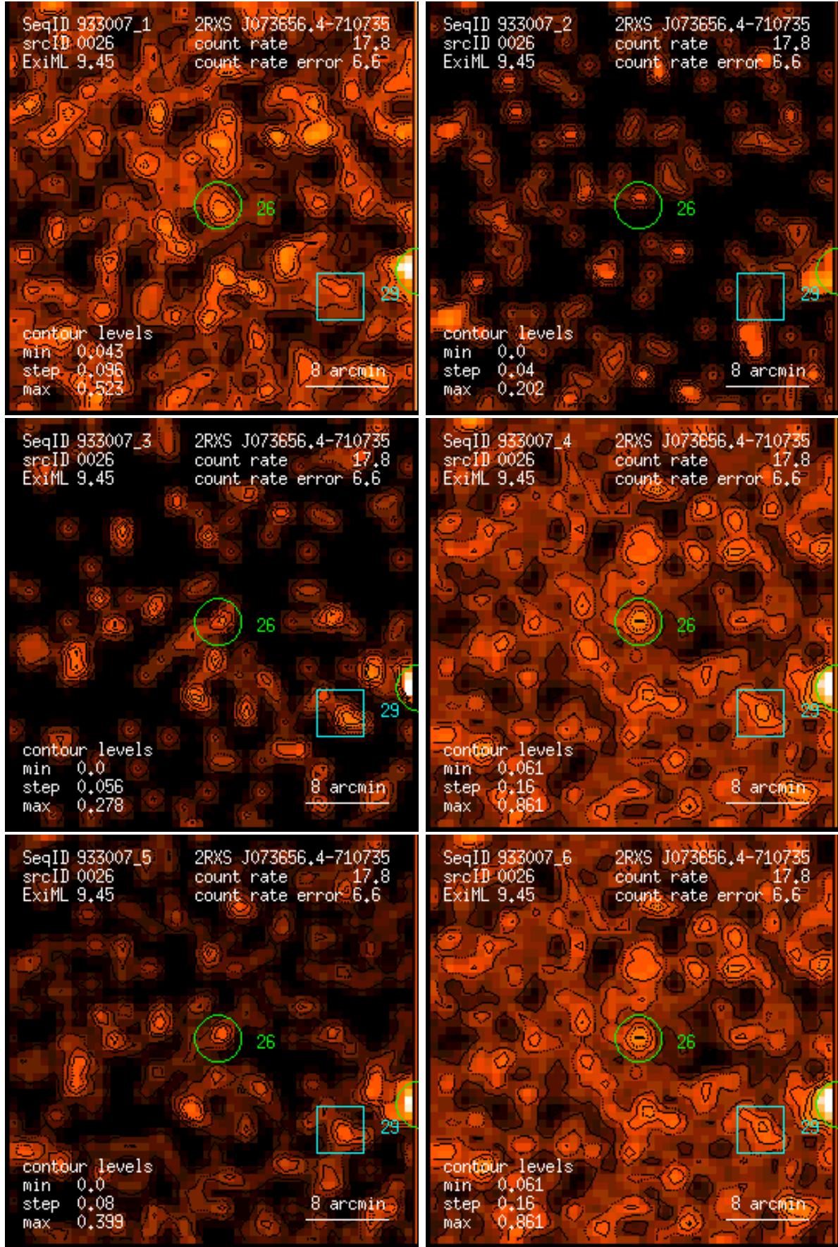
Figure 26: RASS 933007: detection 0026: band rate images, Gaussian filter: (1) PSPC channels 11 – 41, (2) 52 – 90, (3) 91 – 201, (4) 11 – 235, (5) 52 – 201, (6) 11 – 201. Broad band rates in counts/ks. Band rate contour levels in counts/ks/arcmin 2 .
