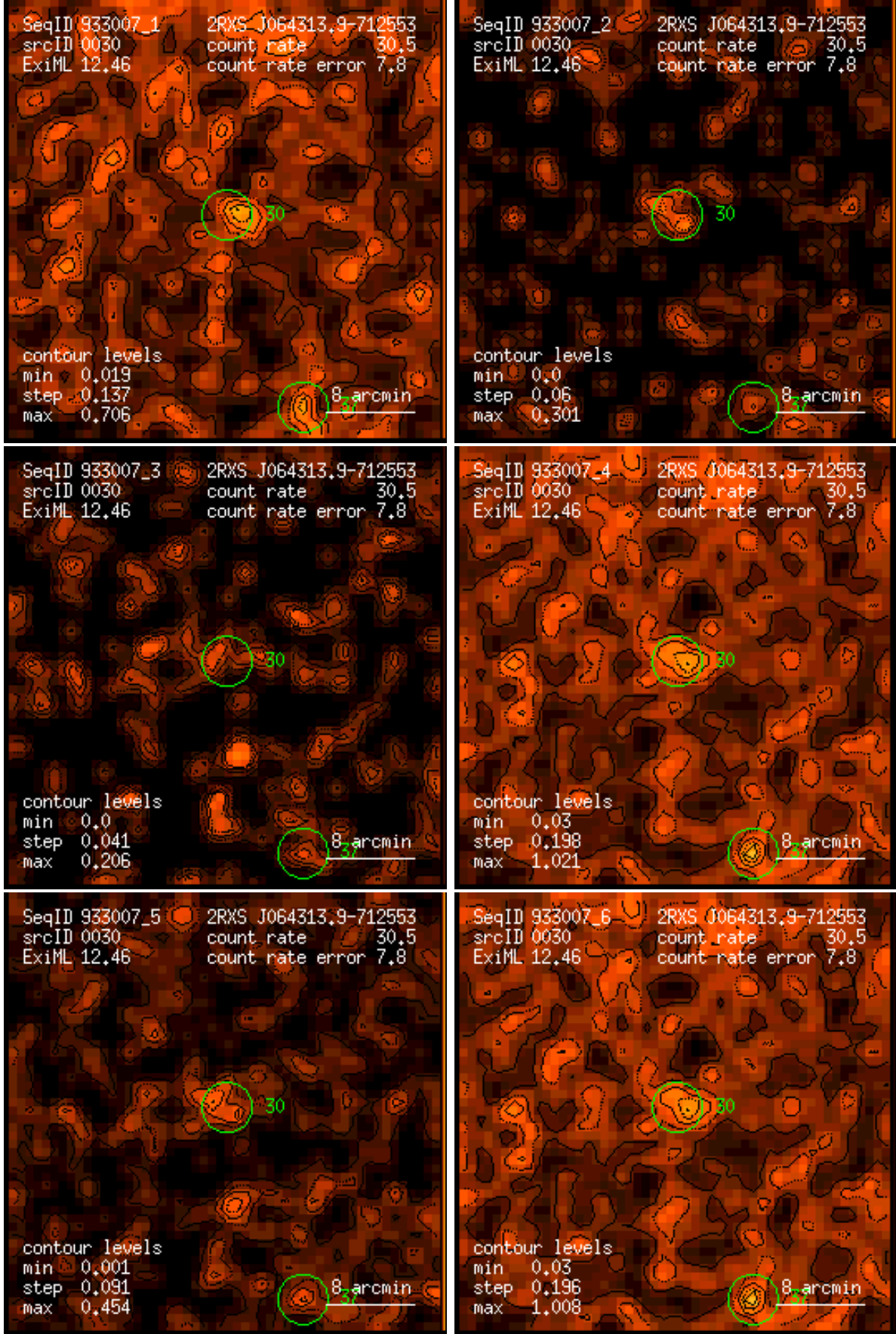
Figure 30: RASS 933007: detection 0030: band rate images, Gaussian filter: (1) PSPC channels 11 – 41, (2) 52 – 90, (3) 91 – 201, (4) 11 – 235, (5) 52 – 201, (6) 11 – 201. Broad band rates in counts/ks. Band rate contour levels in counts/ks/arcmin 2 .
