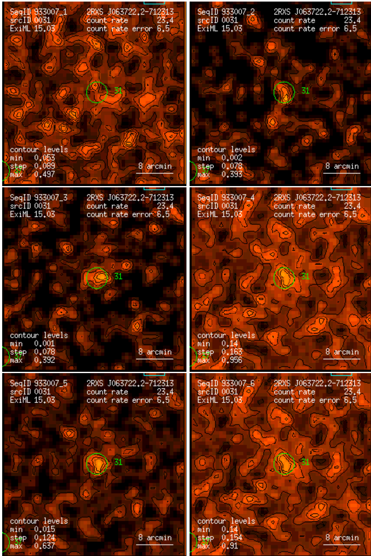
Figure 31: RASS 933007: detection 0031: band rate images, Gaussian filter: (1) PSPC channels 11 – 41, (2) 52 – 90, (3) 91 – 201, (4) 11 – 235, (5) 52 – 201, (6) 11 – 201. Broad band rates in counts/ks. Band rate contour levels in counts/ks/arcmin 2 .
