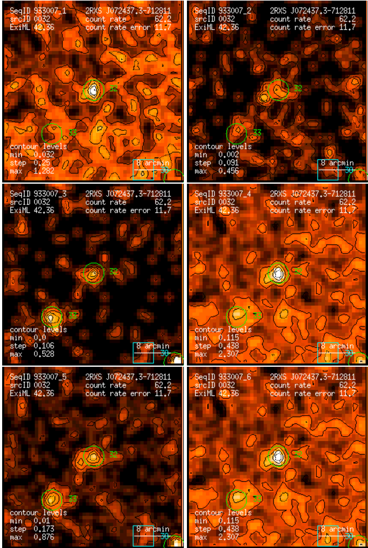
Figure 32: RASS 933007: detection 0032: band rate images, Gaussian filter: (1) PSPC channels 11 – 41, (2) 52 – 90, (3) 91 – 201, (4) 11 – 235, (5) 52 – 201, (6) 11 – 201. Broad band rates in counts/ks. Band rate contour levels in counts/ks/arcmin 2 .
